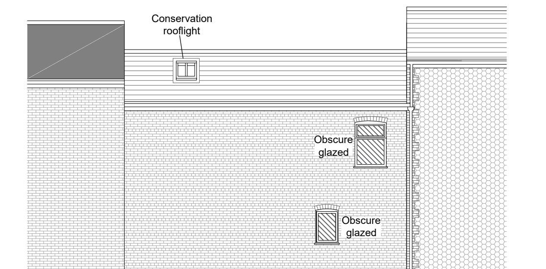
Rear Elevation
