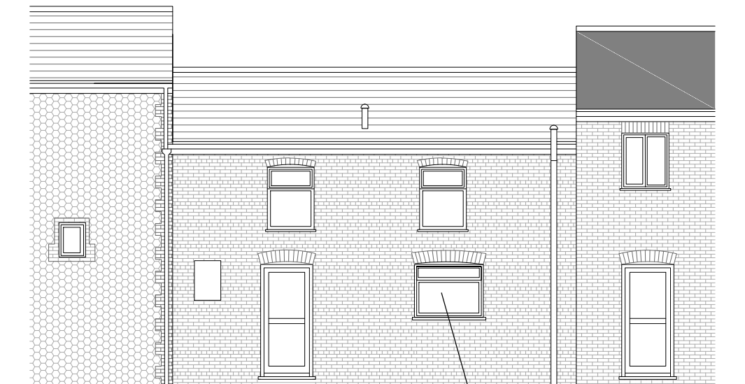
Front Elevation
