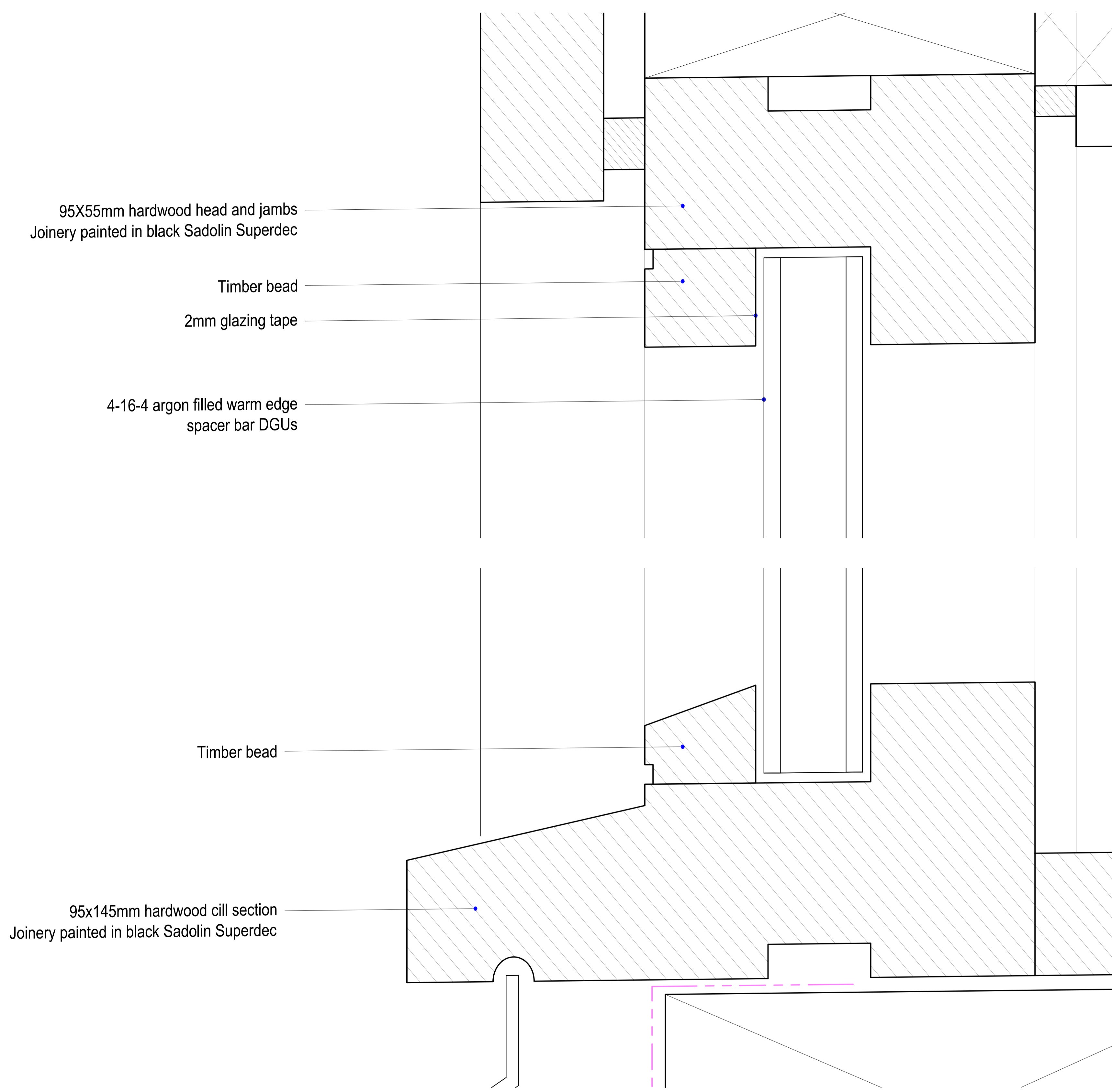
2 / The Garage - Window Section 1:1 at A3
