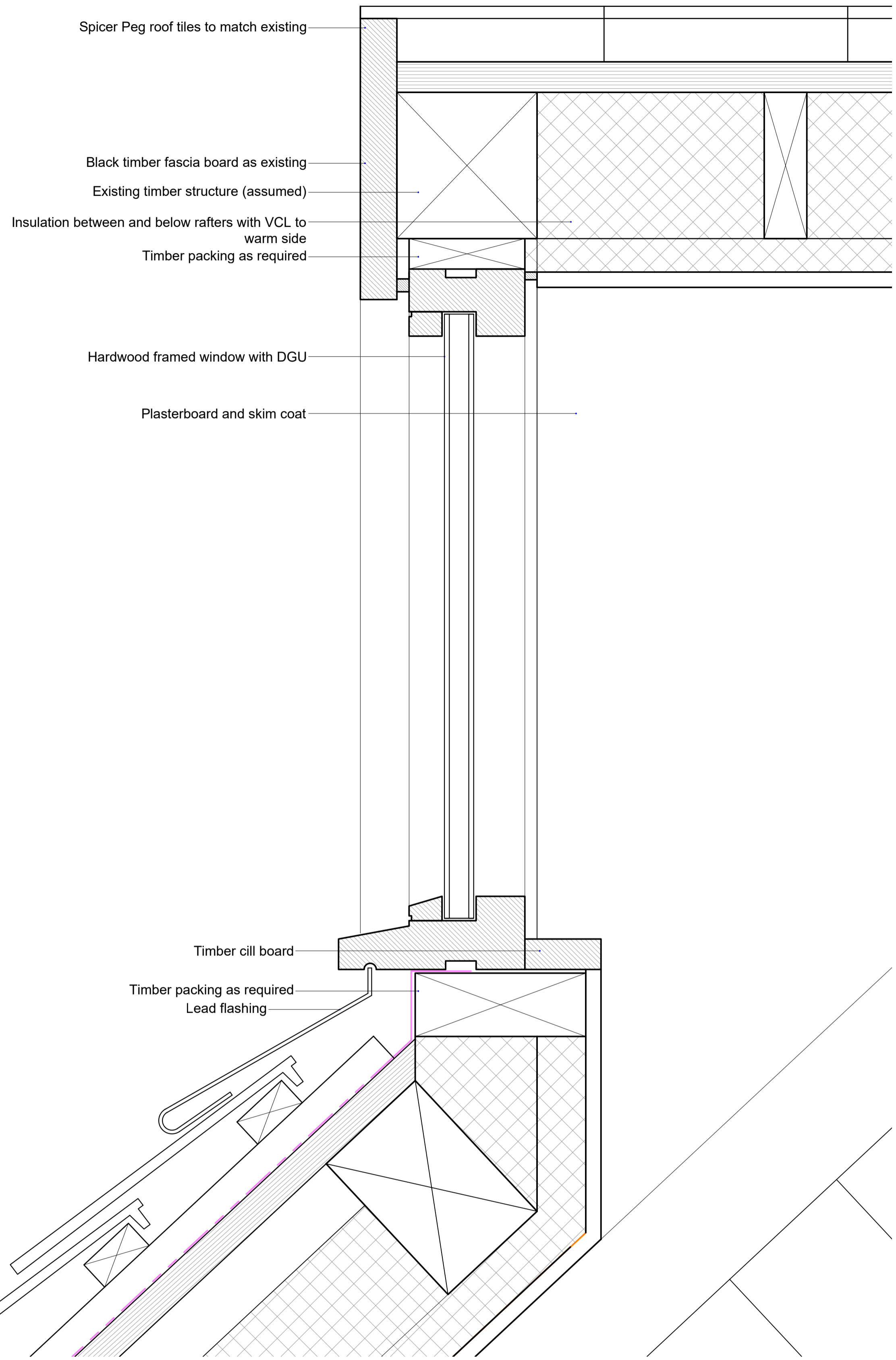
1 / The Garage - Window Detail 1:5 at A3
