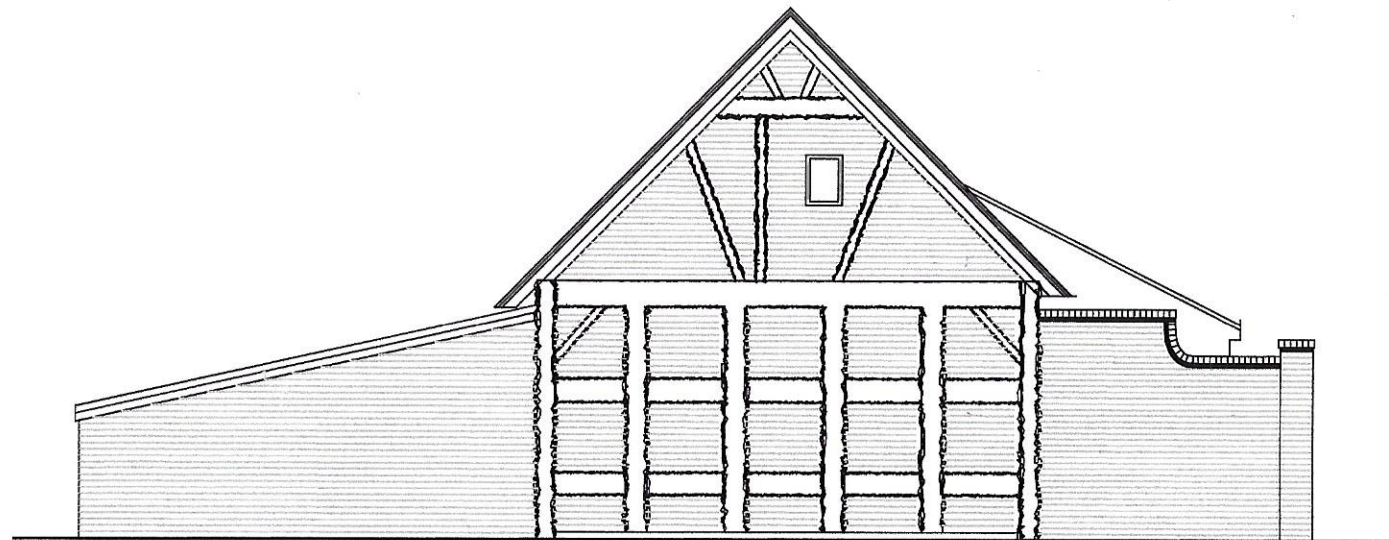
West Elevation. 1:100.
