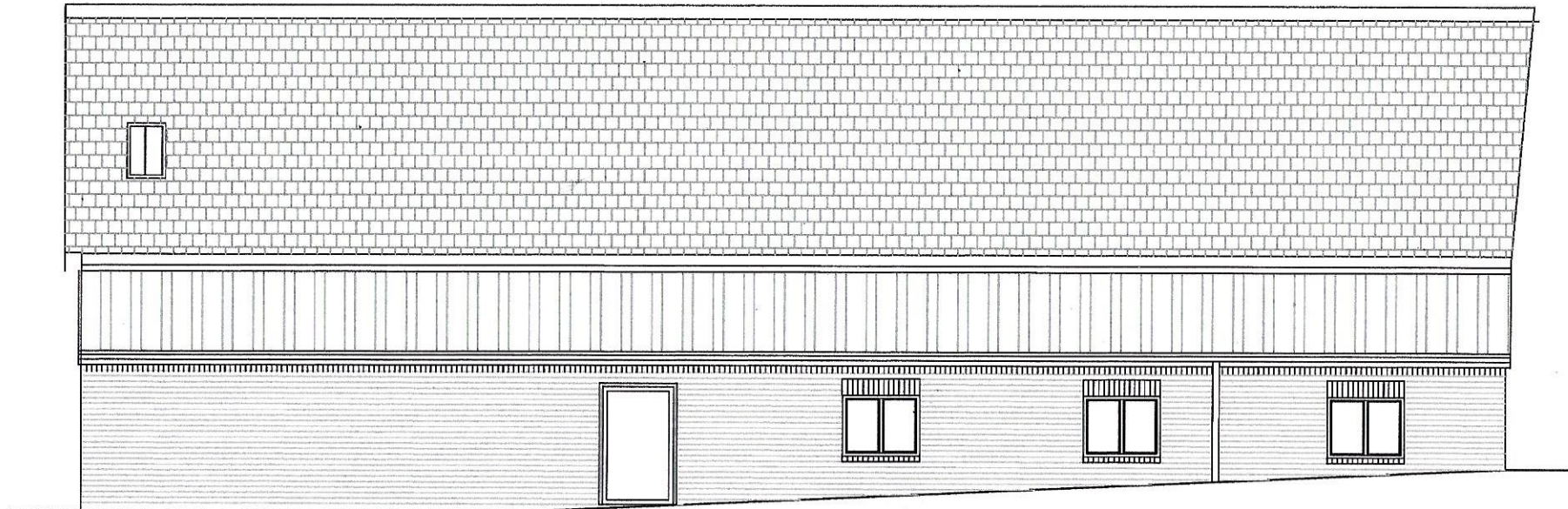
North Elevation. 1:100.
