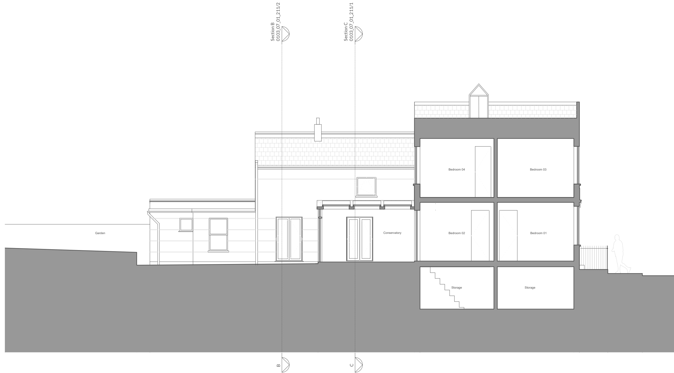
1) PROPOSED - SECTION A / SIDE ELEVATION
