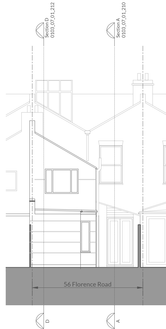
2) PROPOSED - ELEVATION - NORTH / REAR
