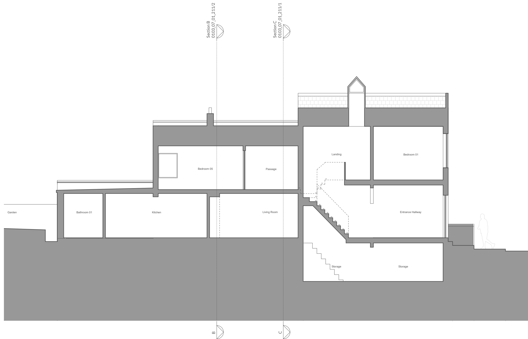
1) PROPOSED - SECTION/ELEVATION D-D
