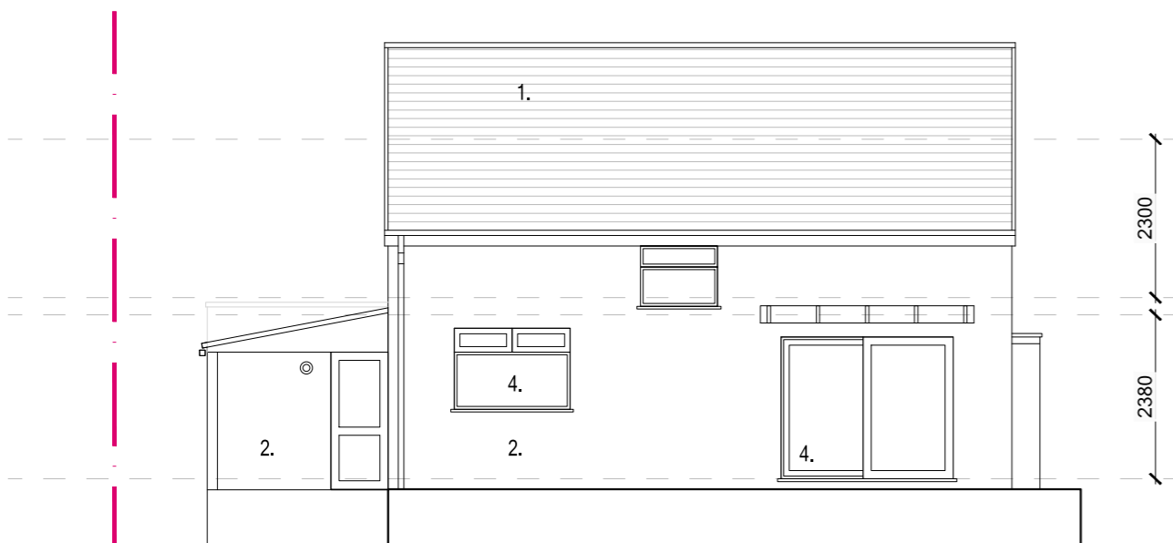
3 EXISTING REAR (NORTH-WEST) ELEVATION (10)03 1:100
