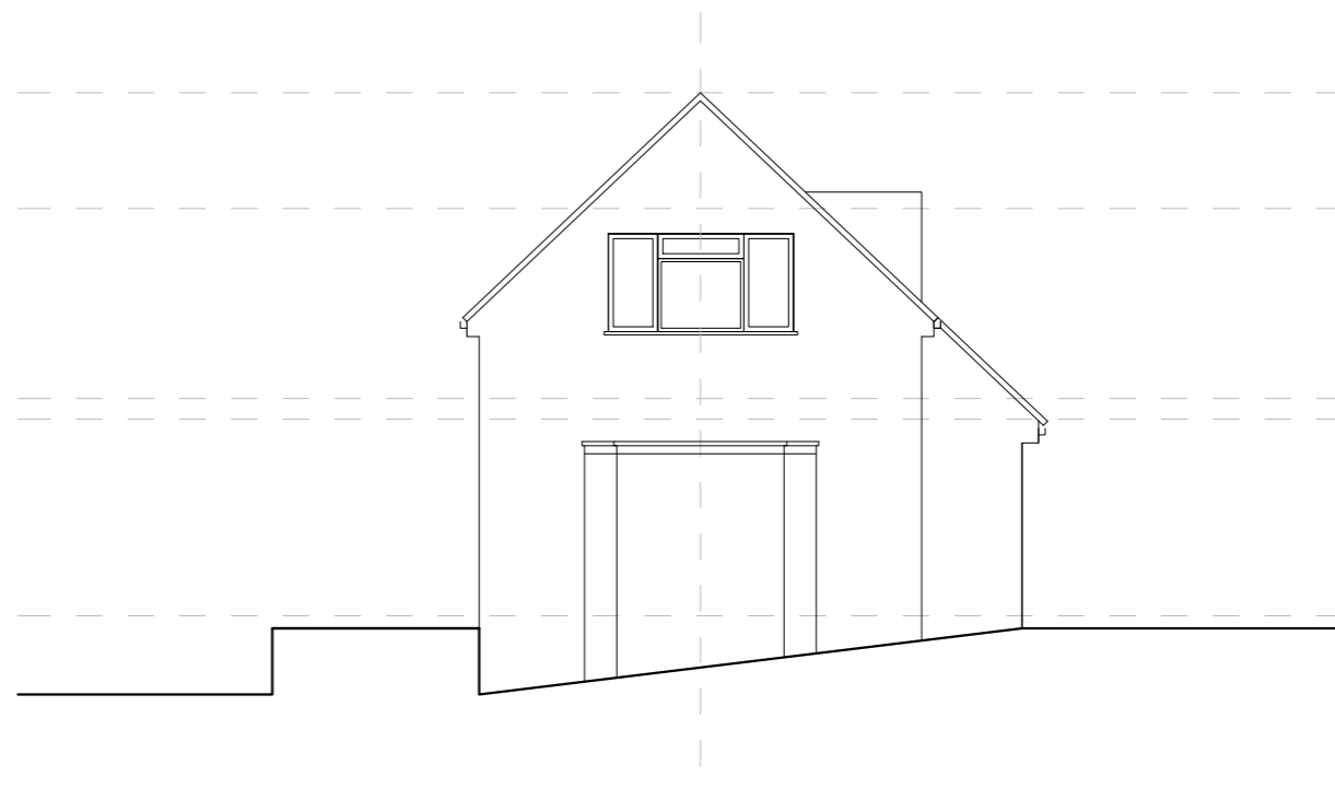
4 EXISTING SIDE (NORTH-EAST) ELEVATION (10)03 1:100
