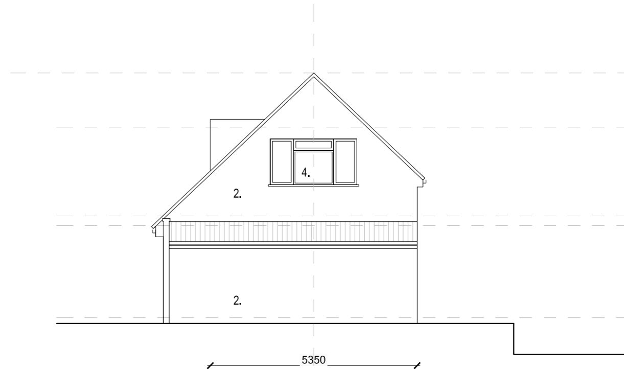
1 EXISTING SIDE (SOUTH-WEST) ELEVATION (10)03 1:100
