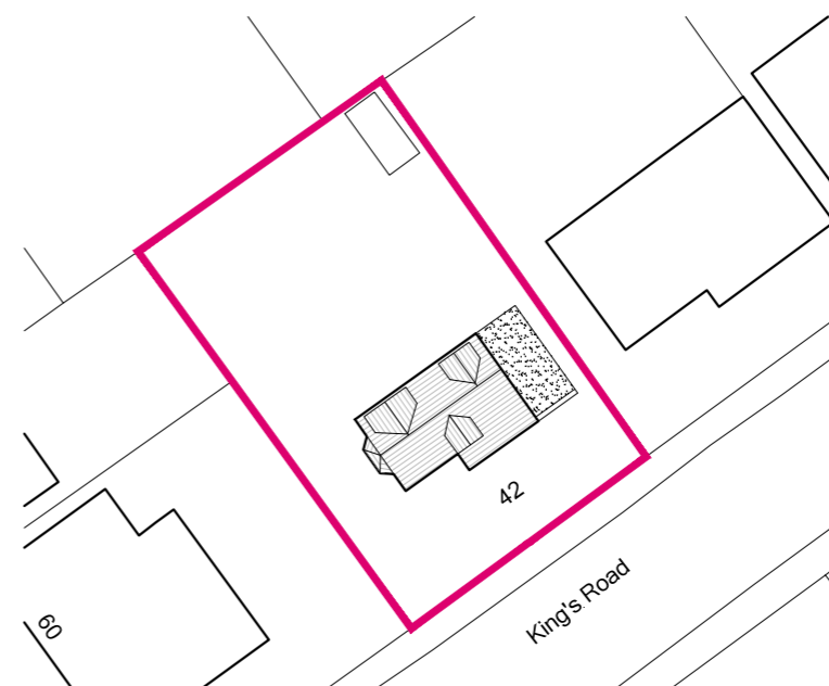
3 PROPOSED BLOCK PLAN (10)01 1:500
