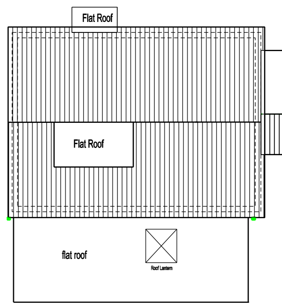
Roof Plan
