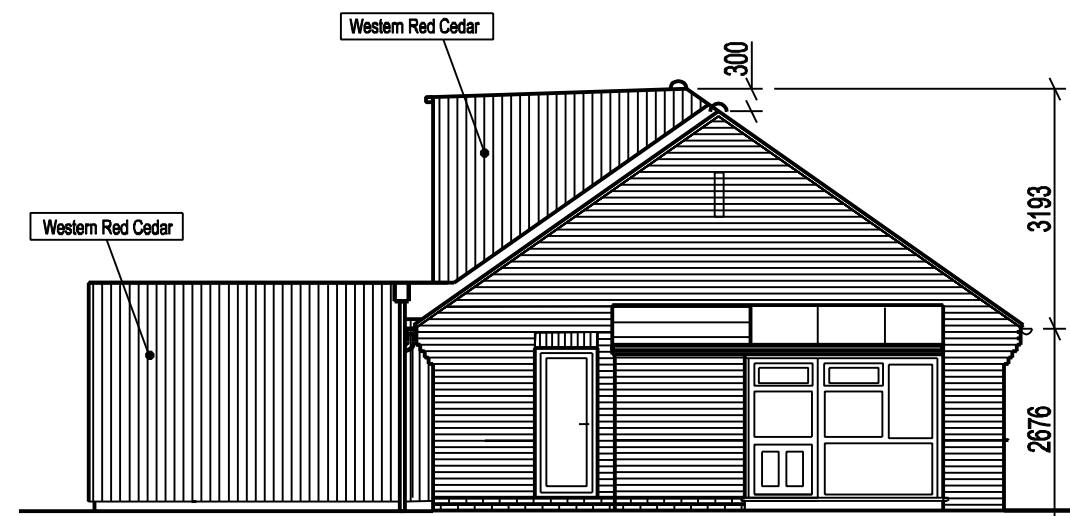
Proposed Side Elevation- South
