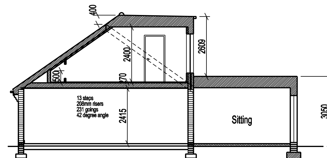
Proposed Section
