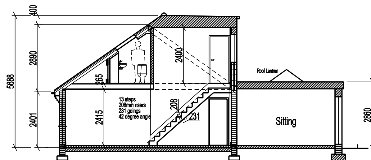
Proposed Section
