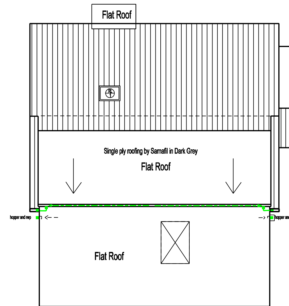
Roof Plan
