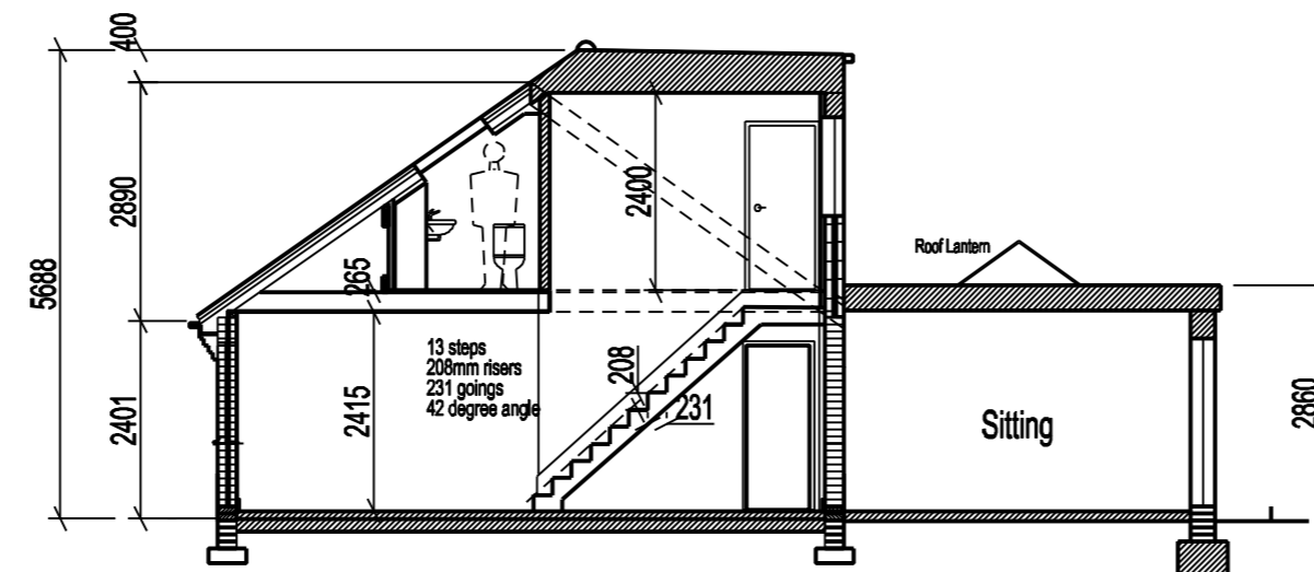
Proposed Section
