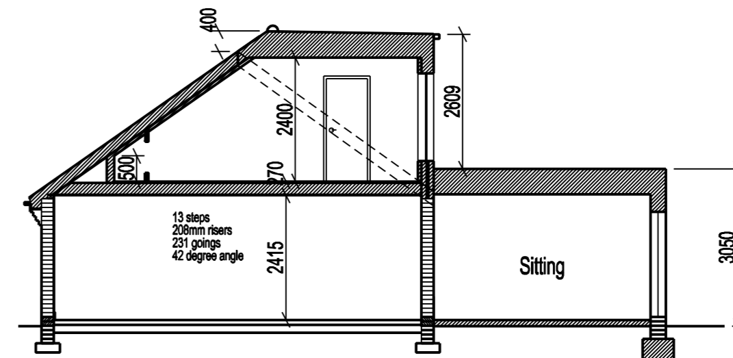
Proposed Section
