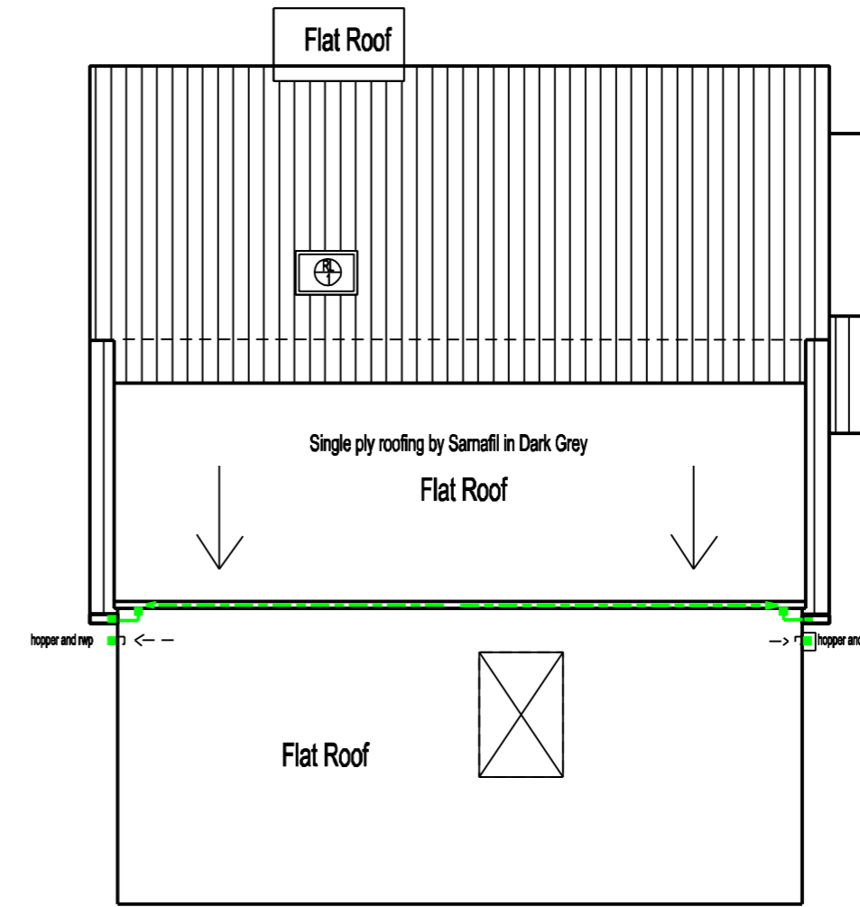
Roof Plan
