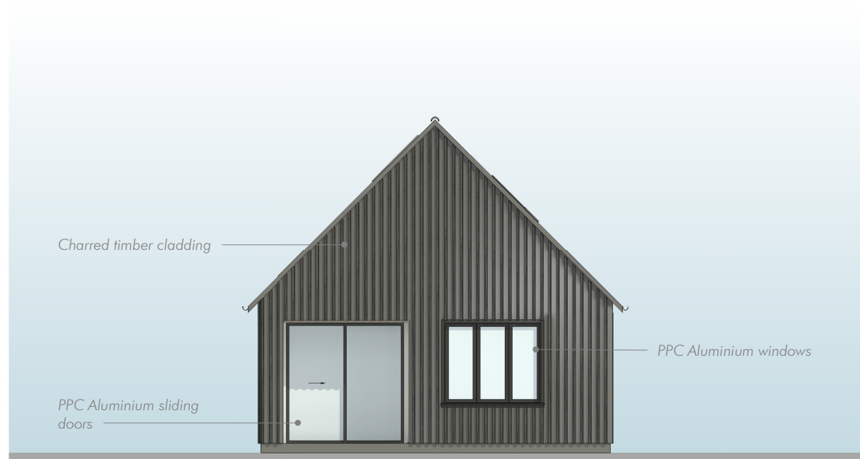
East Elevation 1 : 100
