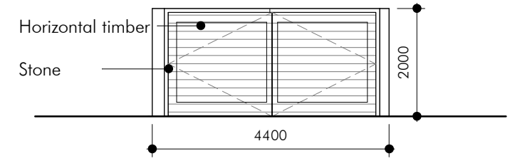
Proposed Entrance Gate Elevation 1 : 100
