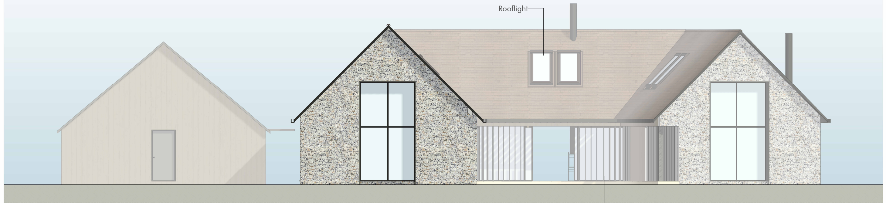
South Elevation 1 : 100
