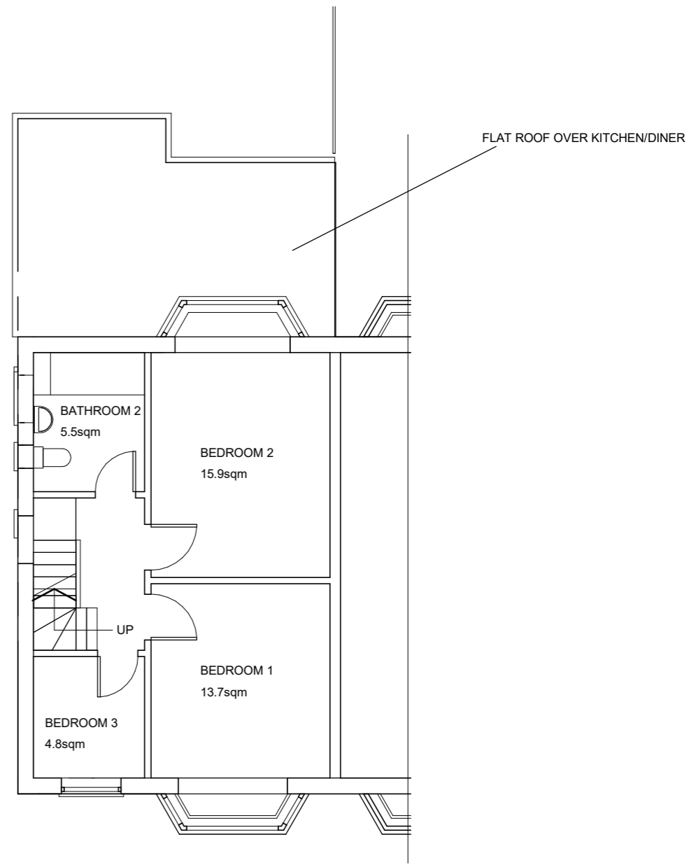
FIRST FLOOR
