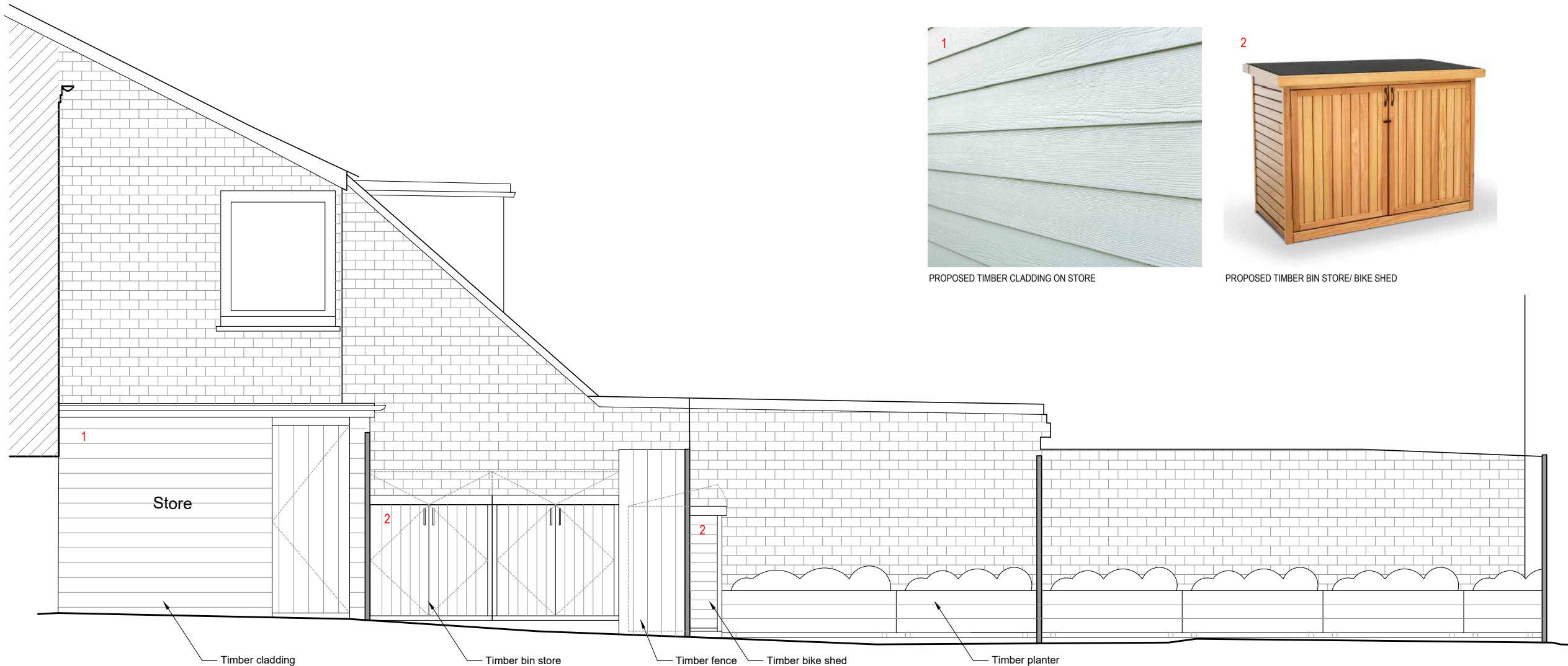
A STORE FRONT ELEVATION
