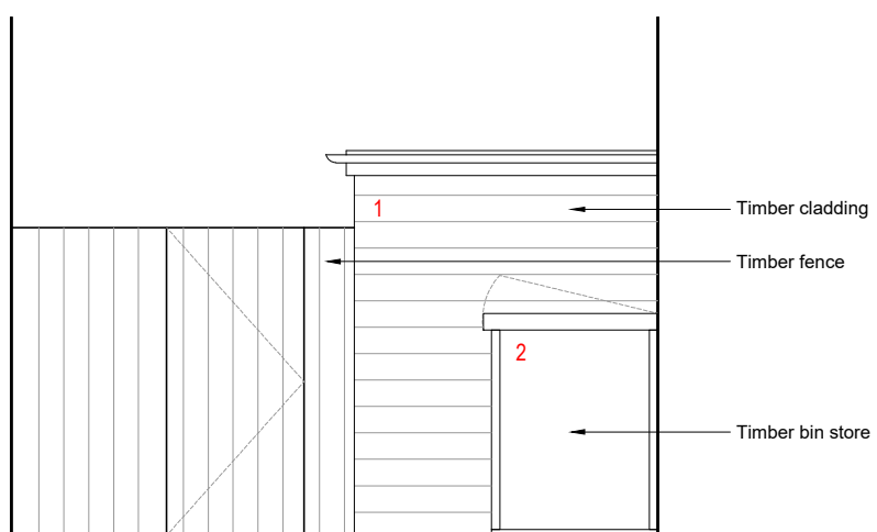
A STORE FRONT ELEVATION
