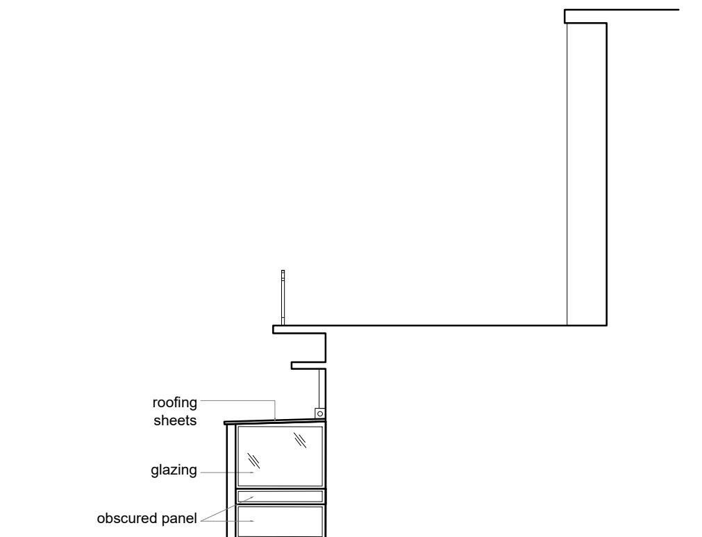
SIDE ELEVATION - 03 Proposed
