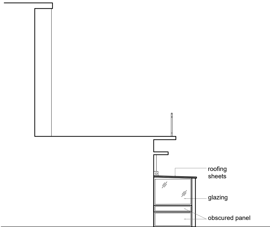
SIDE ELEVATION - 02 Proposed
