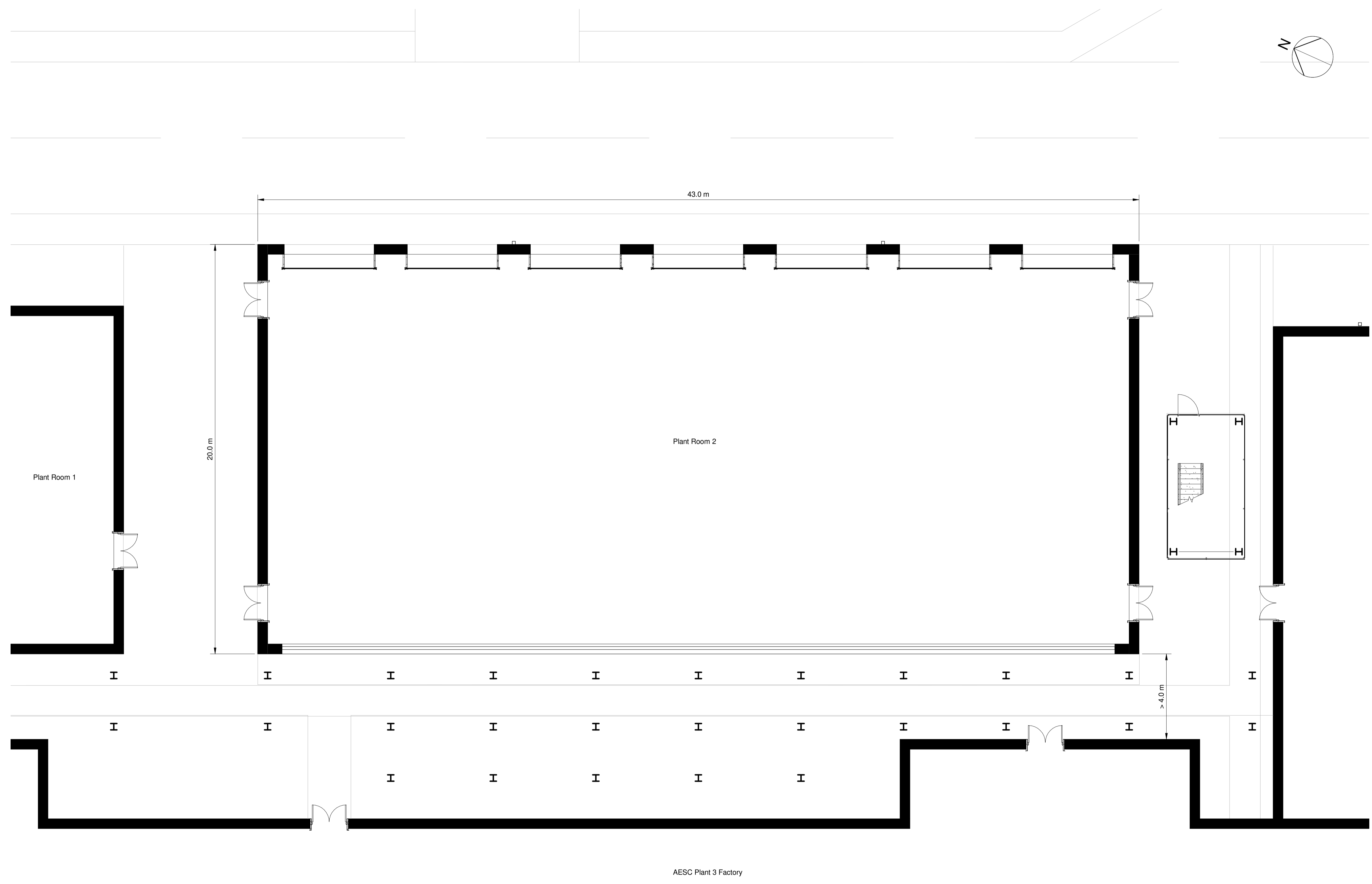
Plant Room 2 - Proposed Plan 1 : 100
