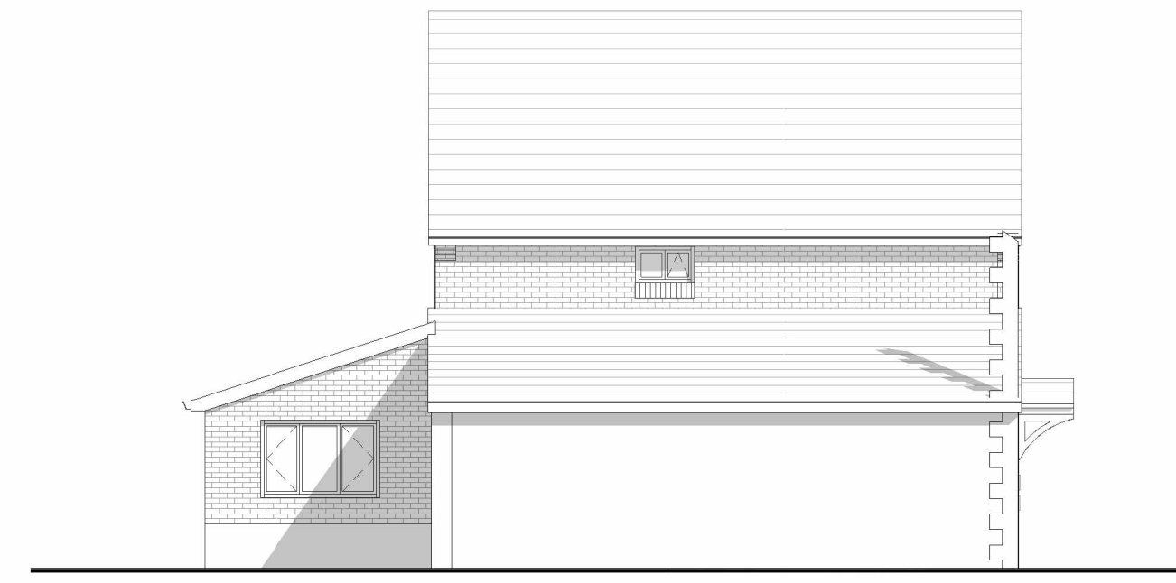
West Elevation 1 : 100
