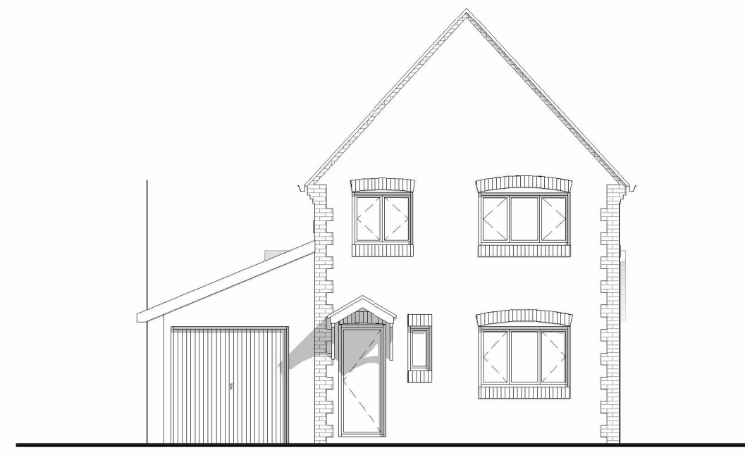
South Elevation 1 : 100
