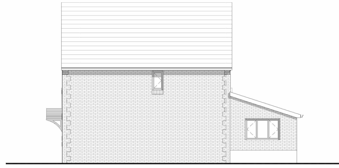
East Elevation 1 : 100
