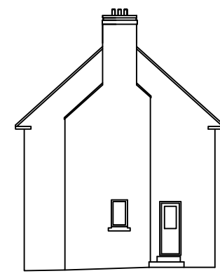
SIDE ELEVATION
