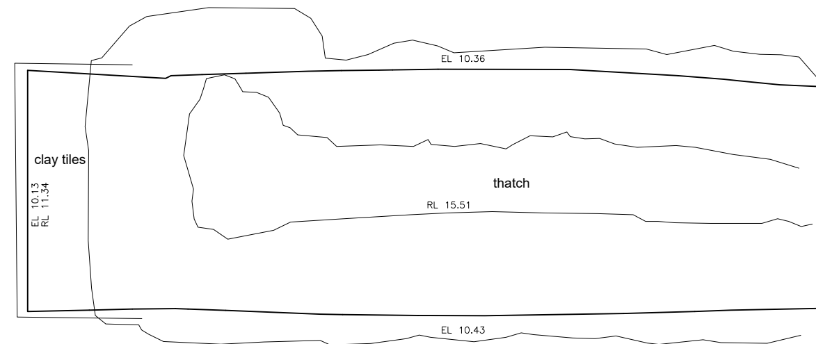
EXISTING ROOF PLAN - 1:100
