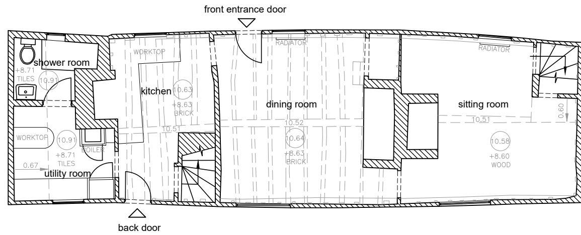
EXISTING GROUND FLOOR PLAN - 1:100
