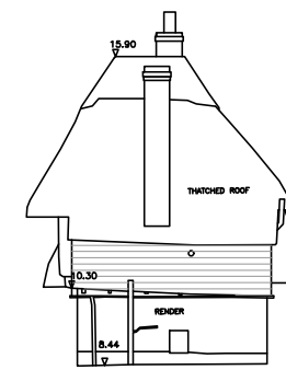
EXISTING SIDE ELEVATION (WEST) - 1:200
