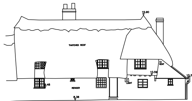
EXISTING FRONT ELEVATION (NORTH) - 1:200
