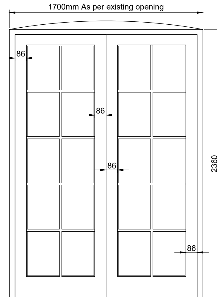
SMALL PANE GLAZED REAR DOOR - FLAT ONE SCALE 1.20 A3
