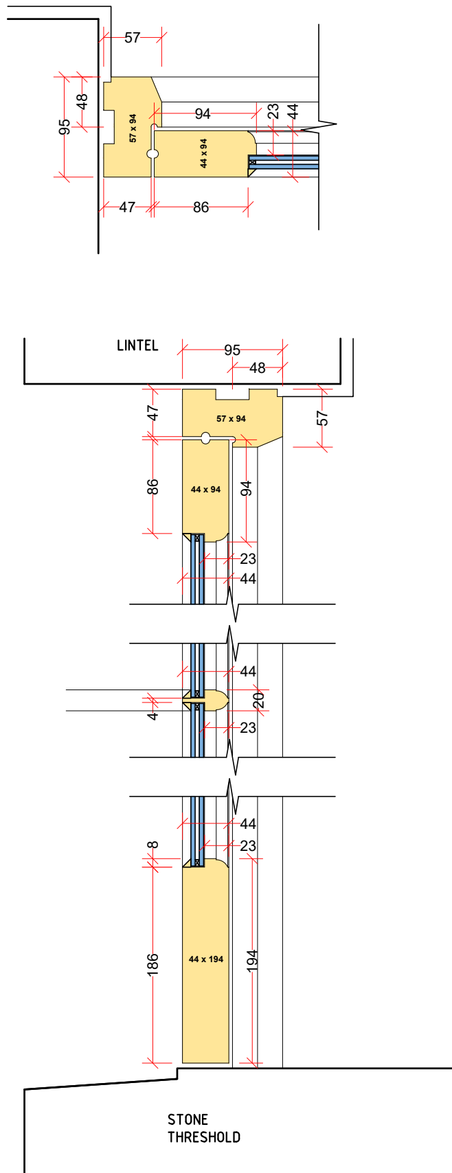
SMALL PANE GLAZED DOOR SECTION SCALE 1.5 A3
