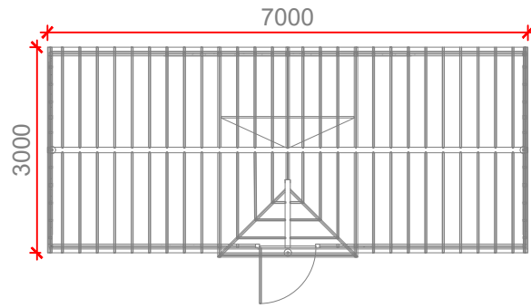
Floor Plan
