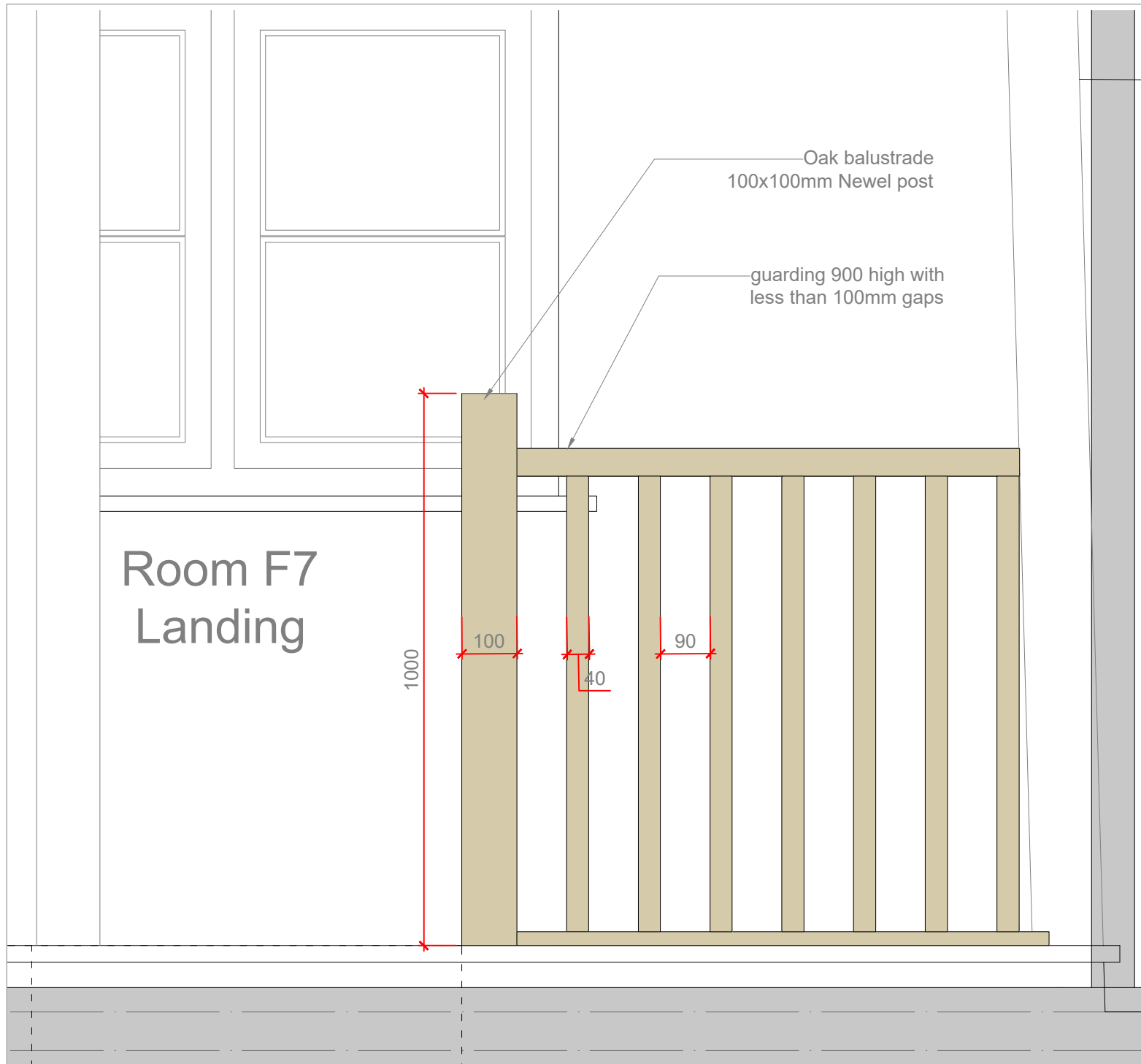
Balustrade elevation 1:10
