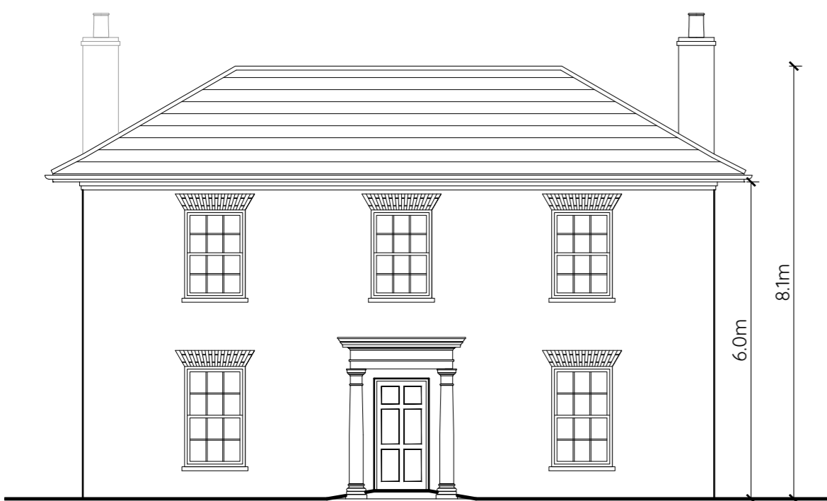
FRONT ELEVATION - North 1:100 Scale @A2 1:141 Scale @A3
