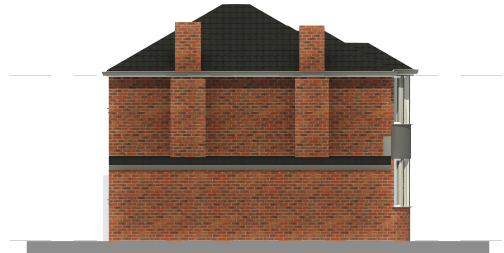
EXISTING AND PROPOSED NORTH ELEVATION 1:100
