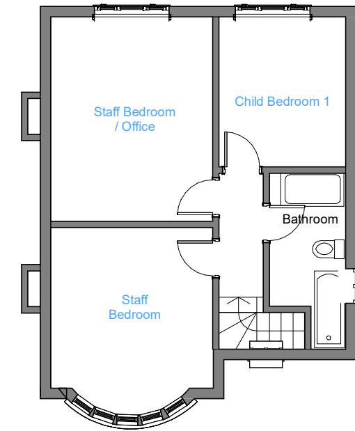
PROPOSED FIRST FLOOR PLAN 1:100
