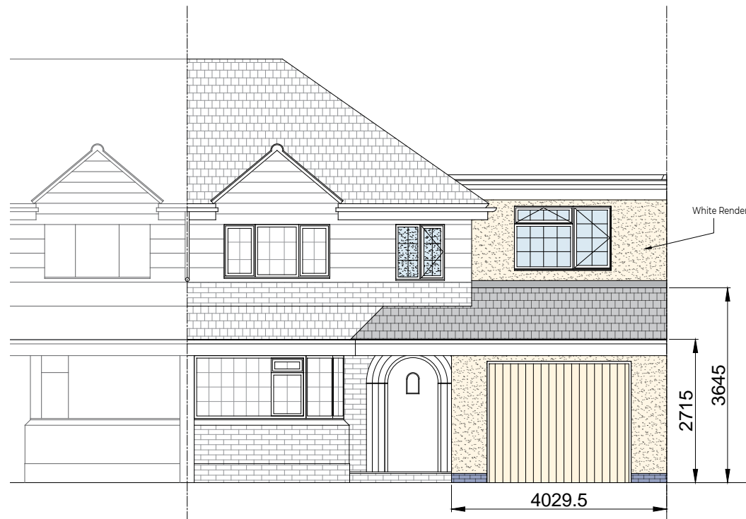
Proposed Front Elevation (East)
