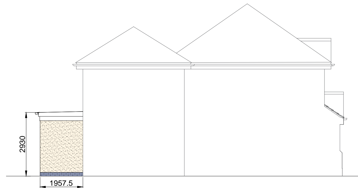
Proposed Side Elevation from No.13 (South)
