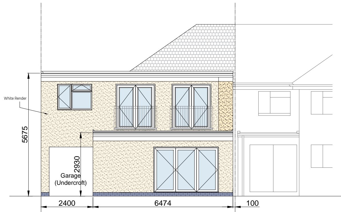
Proposed Rear Elevation (West)
