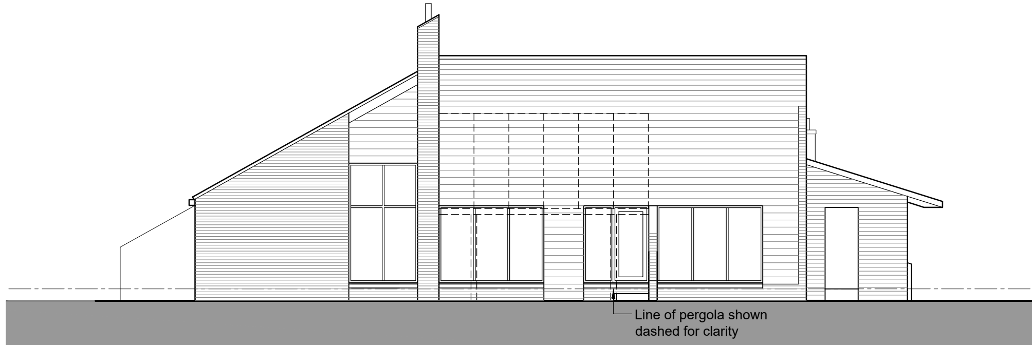
1 East Elevation
