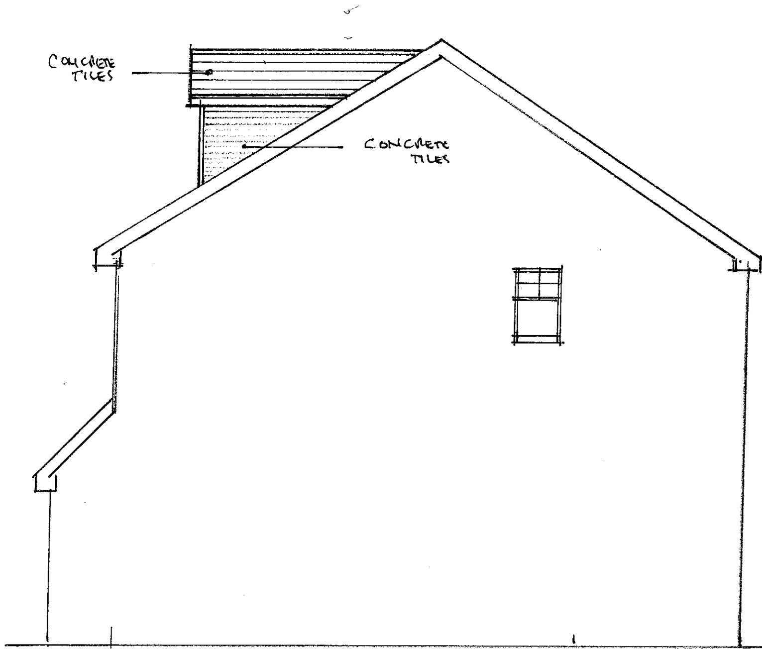
PROPOSED SIDE ELEVATION 1:50 @ A3
