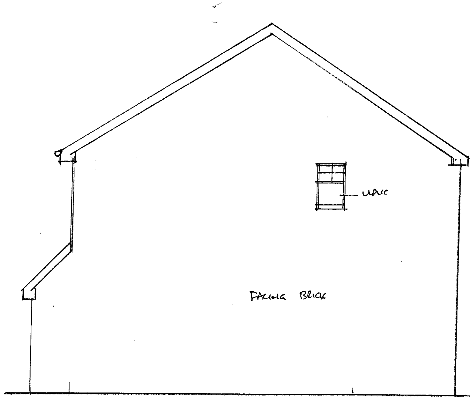
EXISTING SIDE ELEVATION 1:50 @ A3
