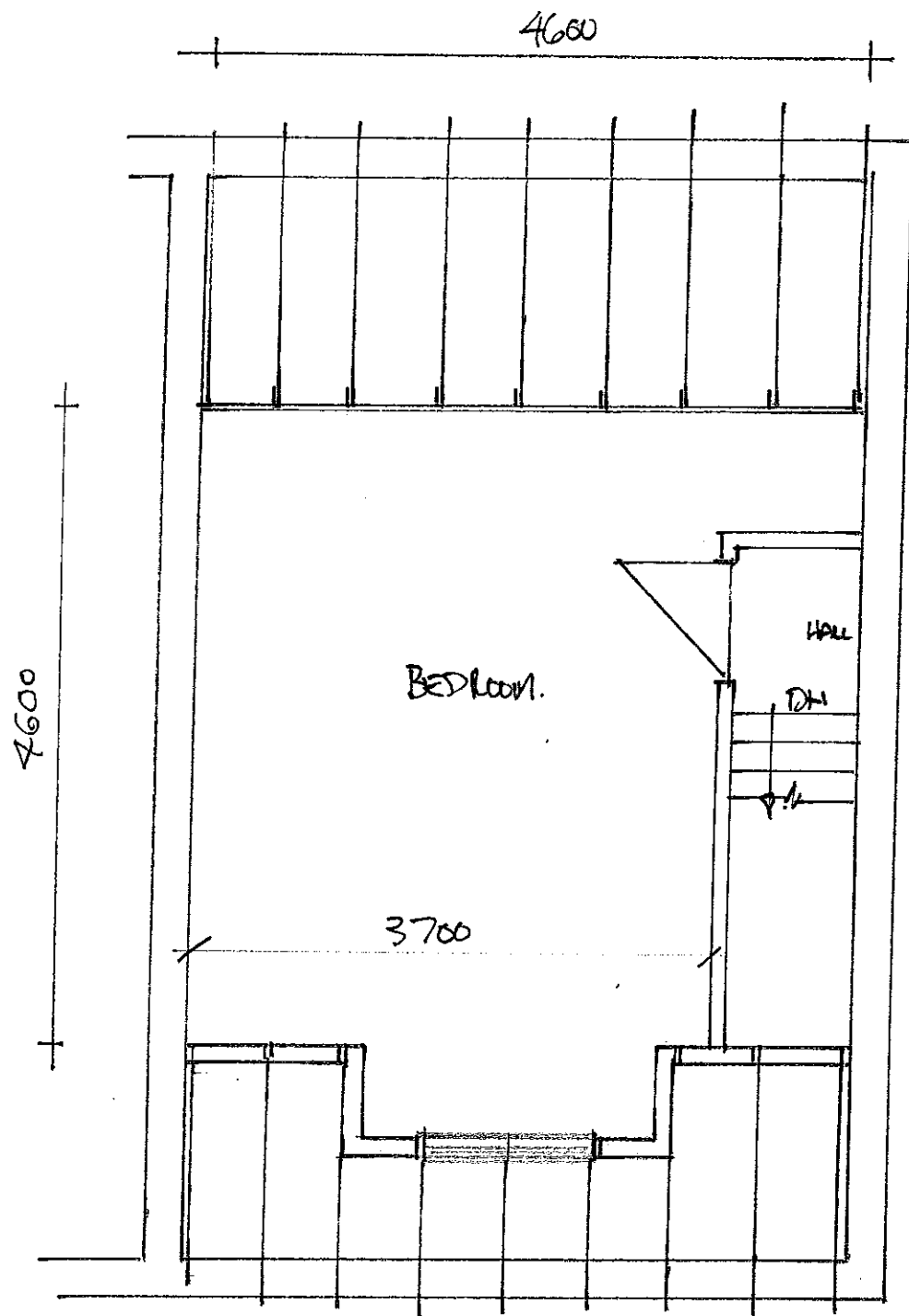
PROPOSED ATTIC LEVEL PLAN 1:50 @ A3
