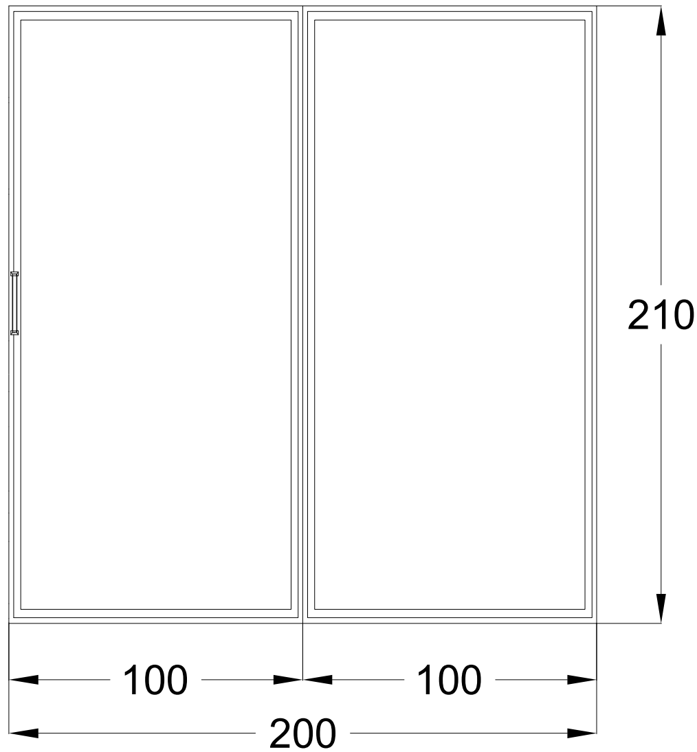
SLIDING DOOR IN UPVC MATERIAL COLOUR RAL 7016
