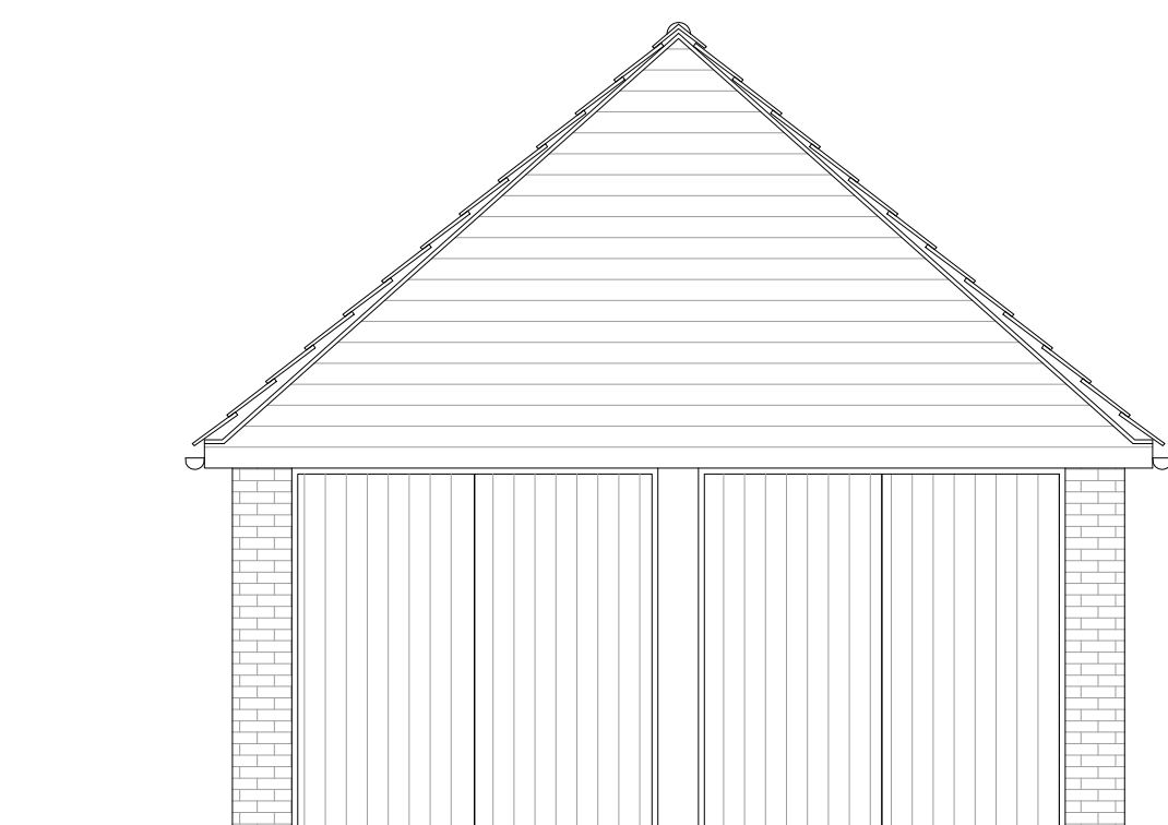
GARAGE FRONT ELEVATION 1:50
