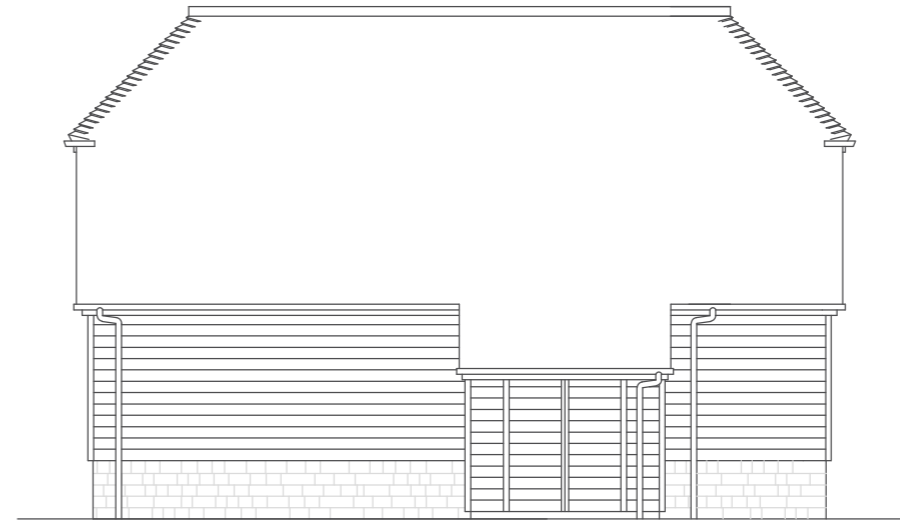
North elevation
