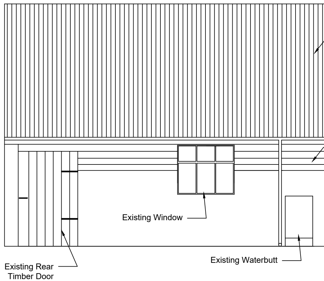
NORTHERN ELEVATION
