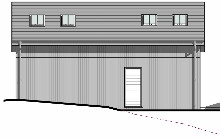
North Elevation 1:100
