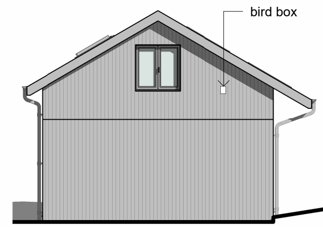
West Elevation 1:100
