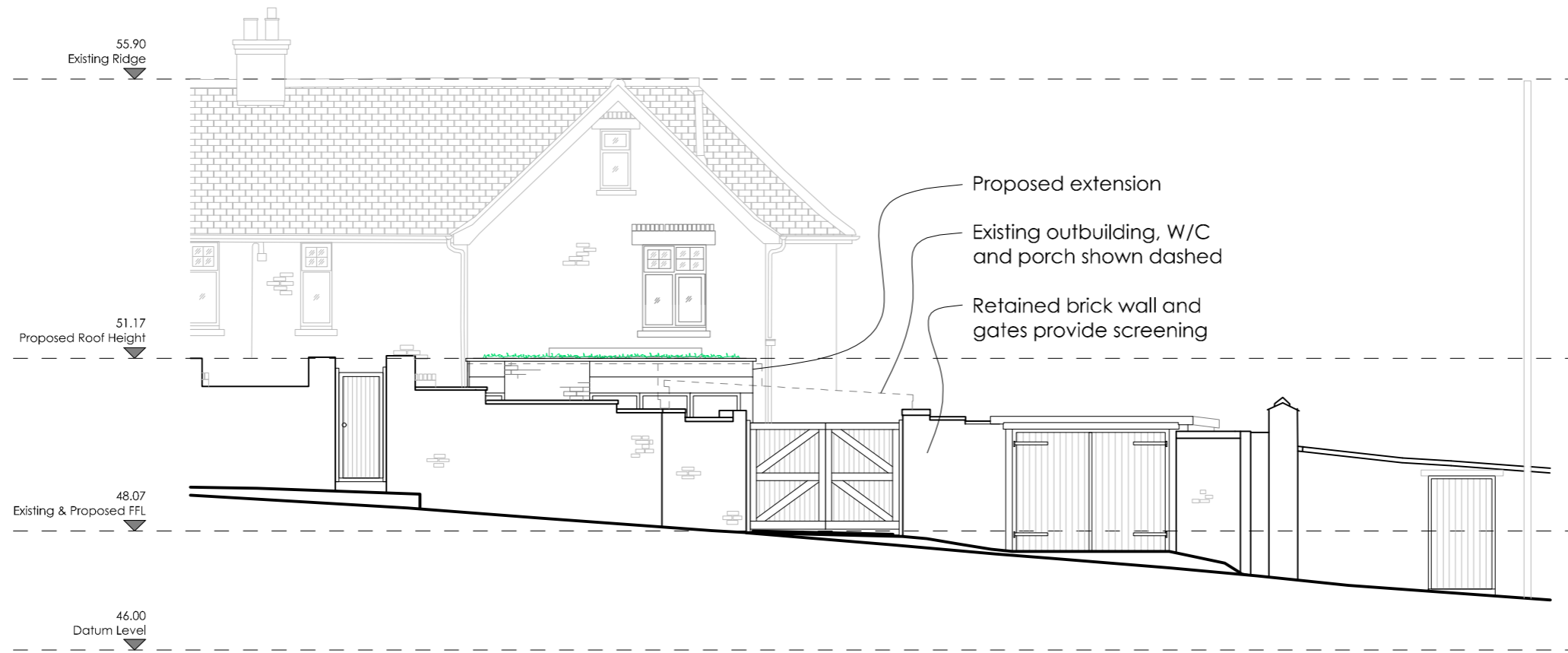
Proposed Street Elevation - Four Mills Lane
