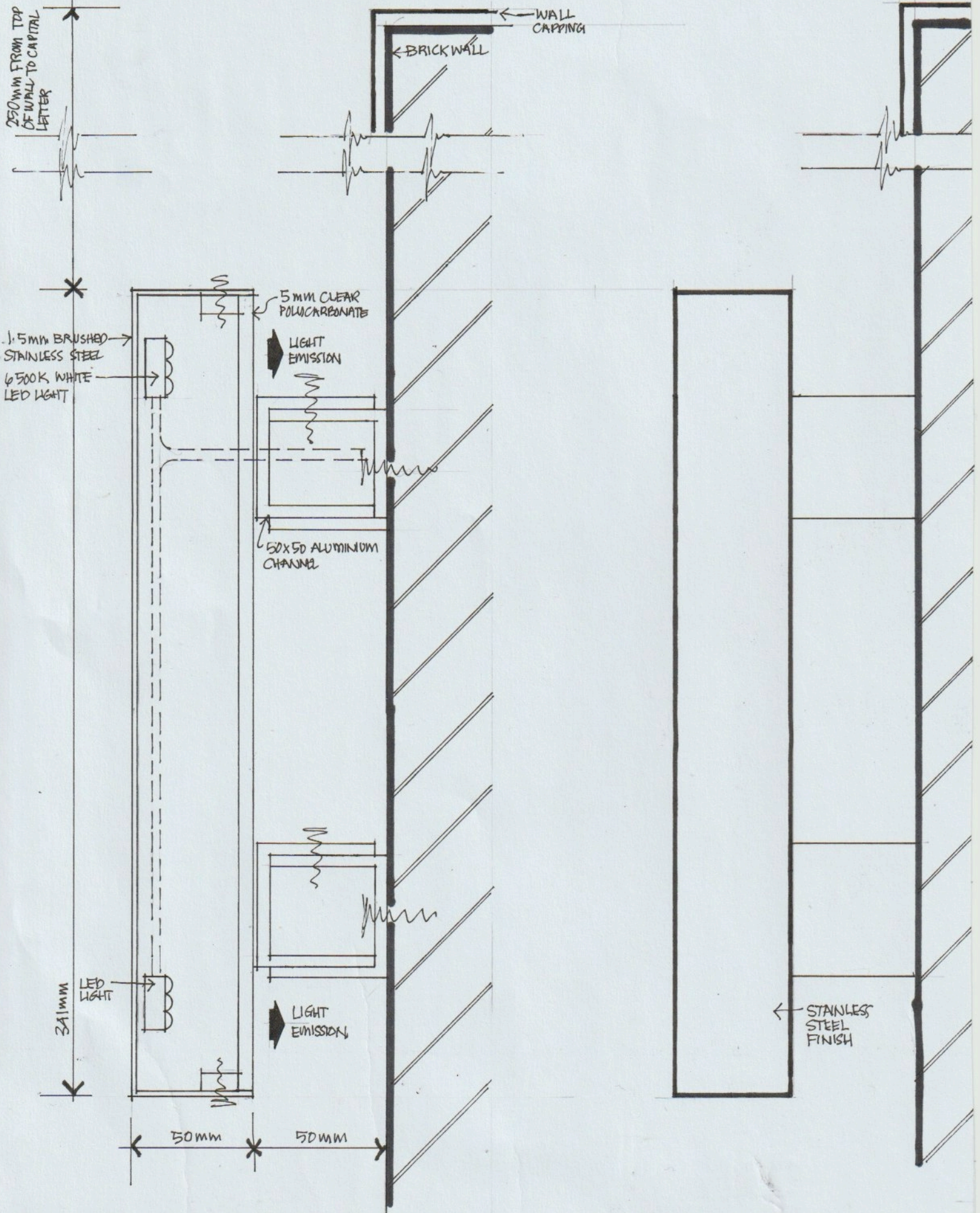
1/2 FULL SIZE SECTION THROUGH SIGN
