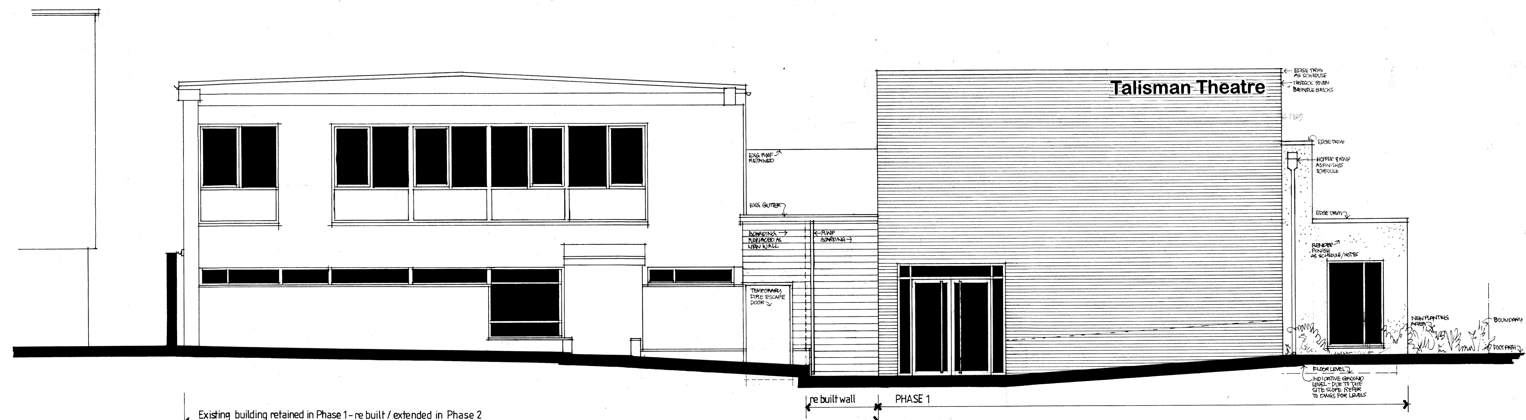
PHASE 1 ELEVATION TO BARROWS LANE 1 / 50
