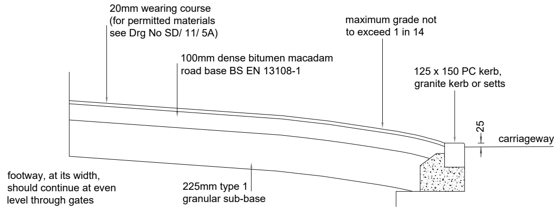
Medium duty - Bituminous
