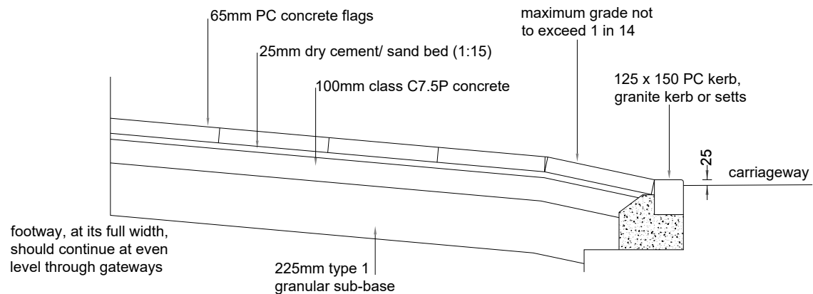
Medium duty - Flags (only permitted where existing footway is in flag construction)
