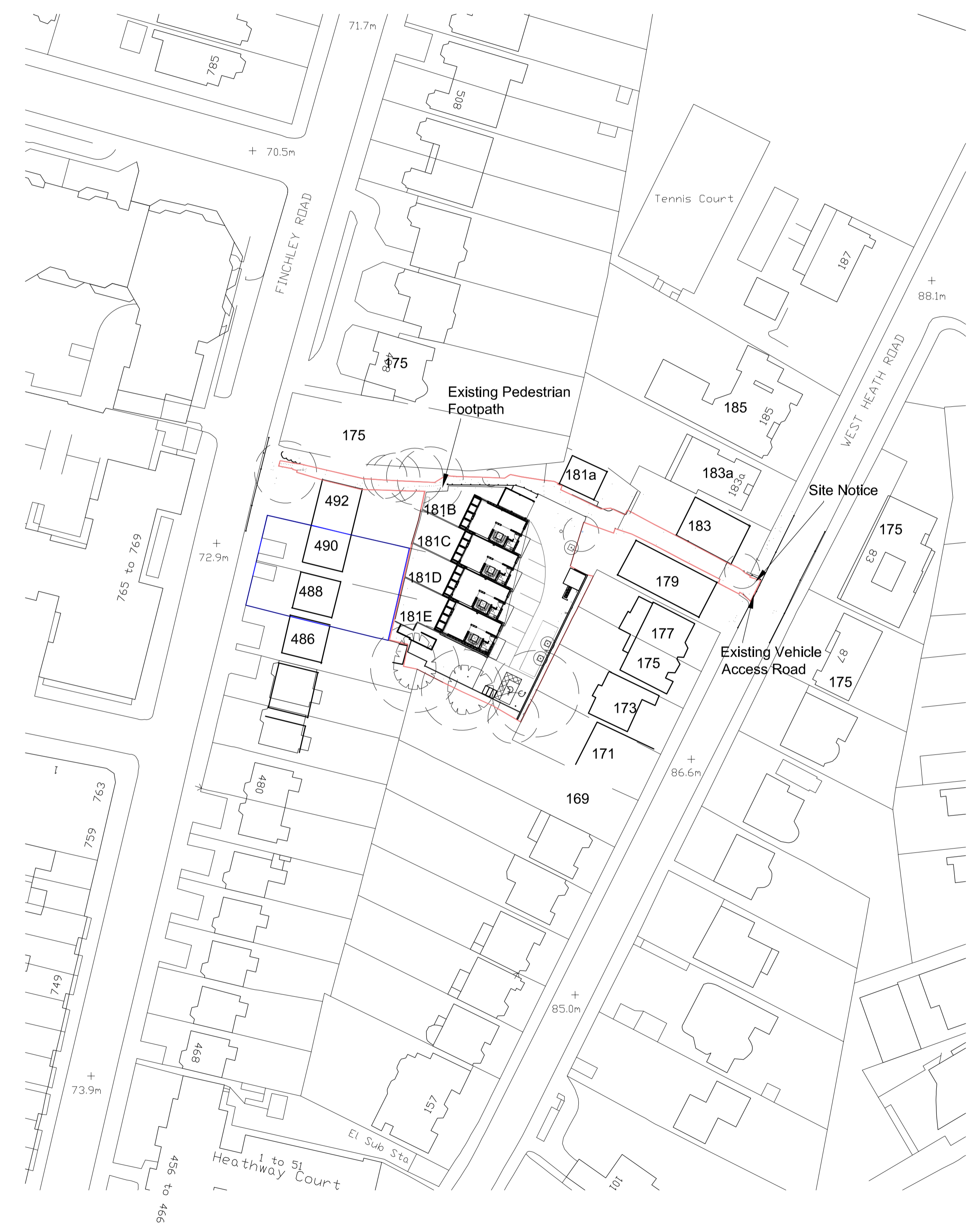
1 Proposed Site Location Plan SCALE 1:1250@A3
