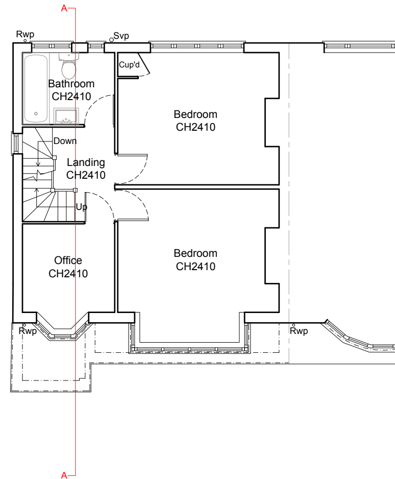
First Floor Plan As Existing 1:100
