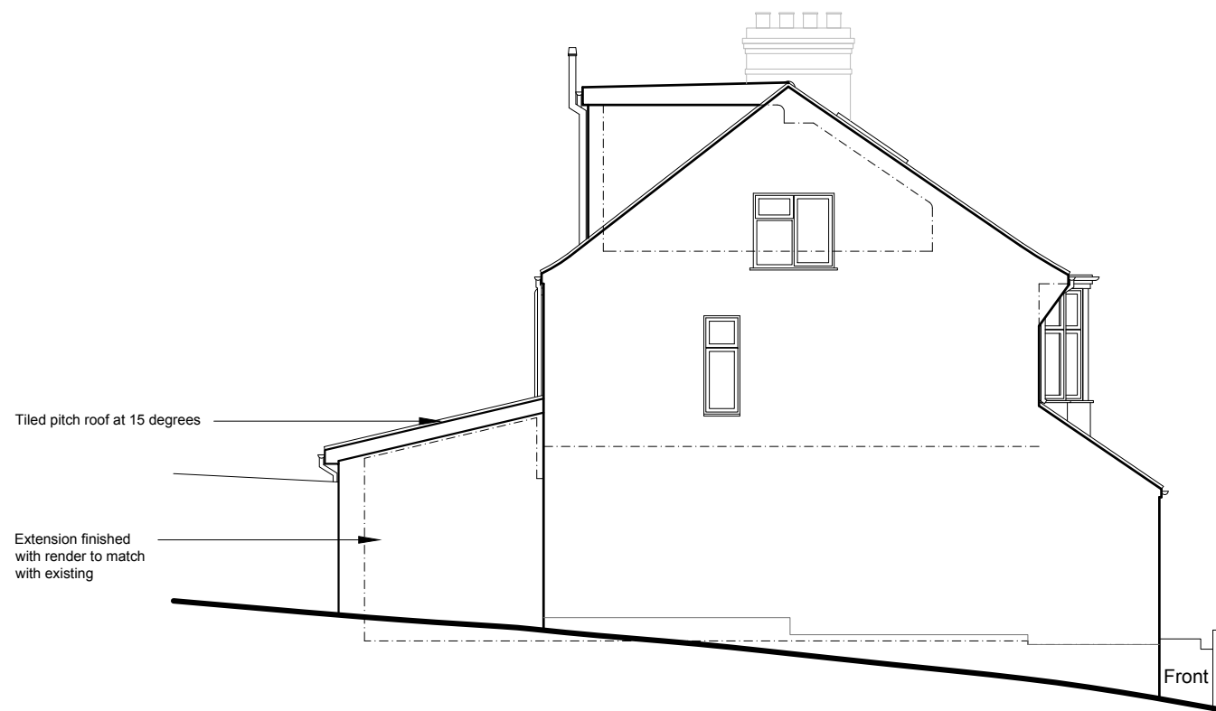
Side Elevation As Proposed 1:100
