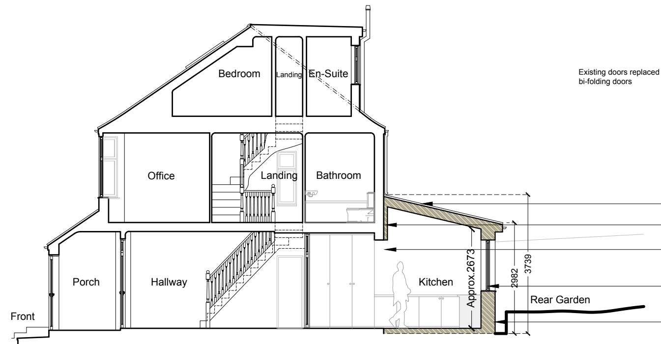
Section A-A As Proposed 1:100
