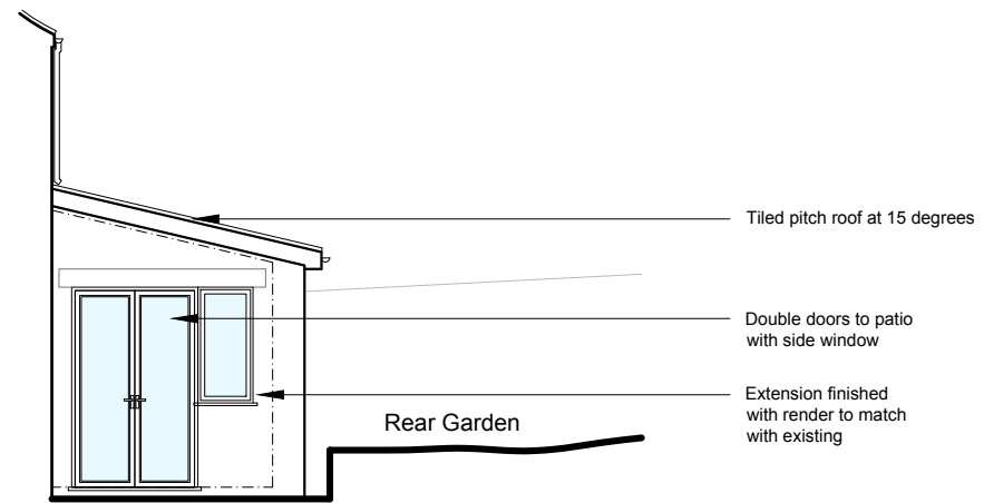
Side Elevation As Proposed 1:100
