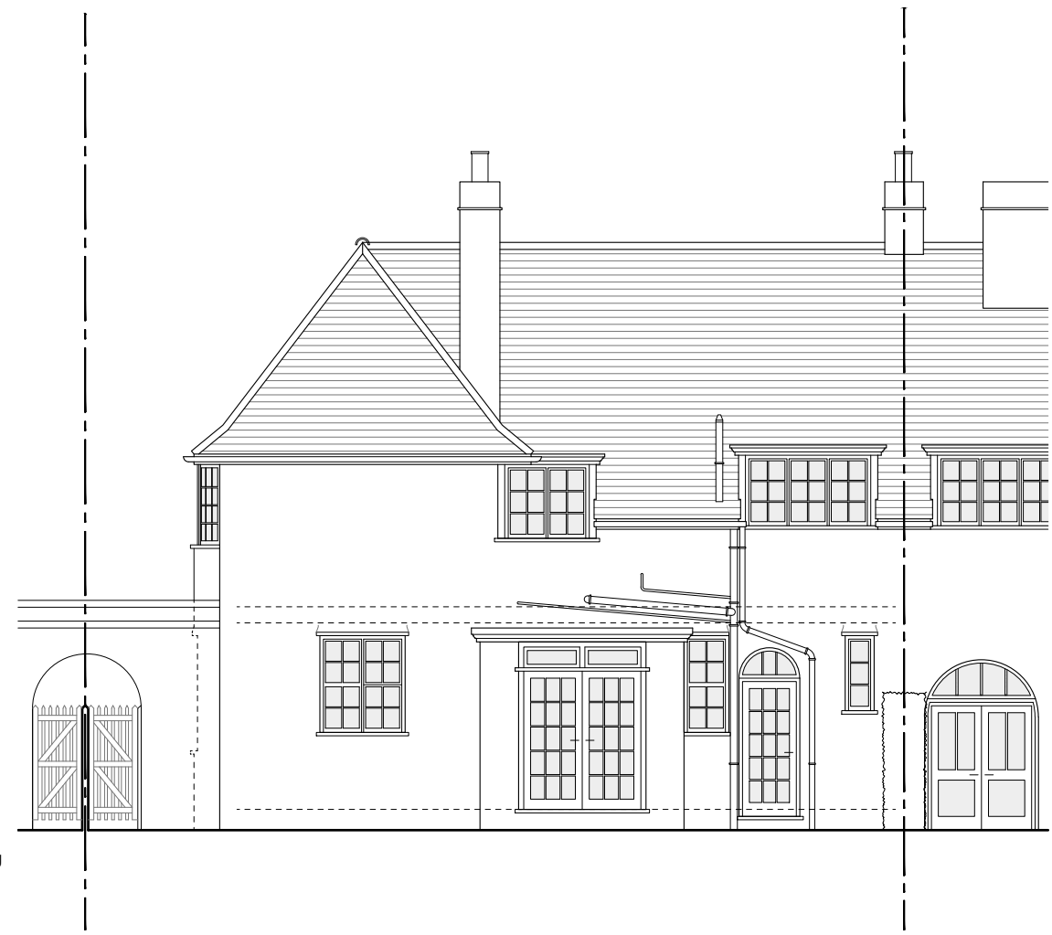
REAR ELEVATION
