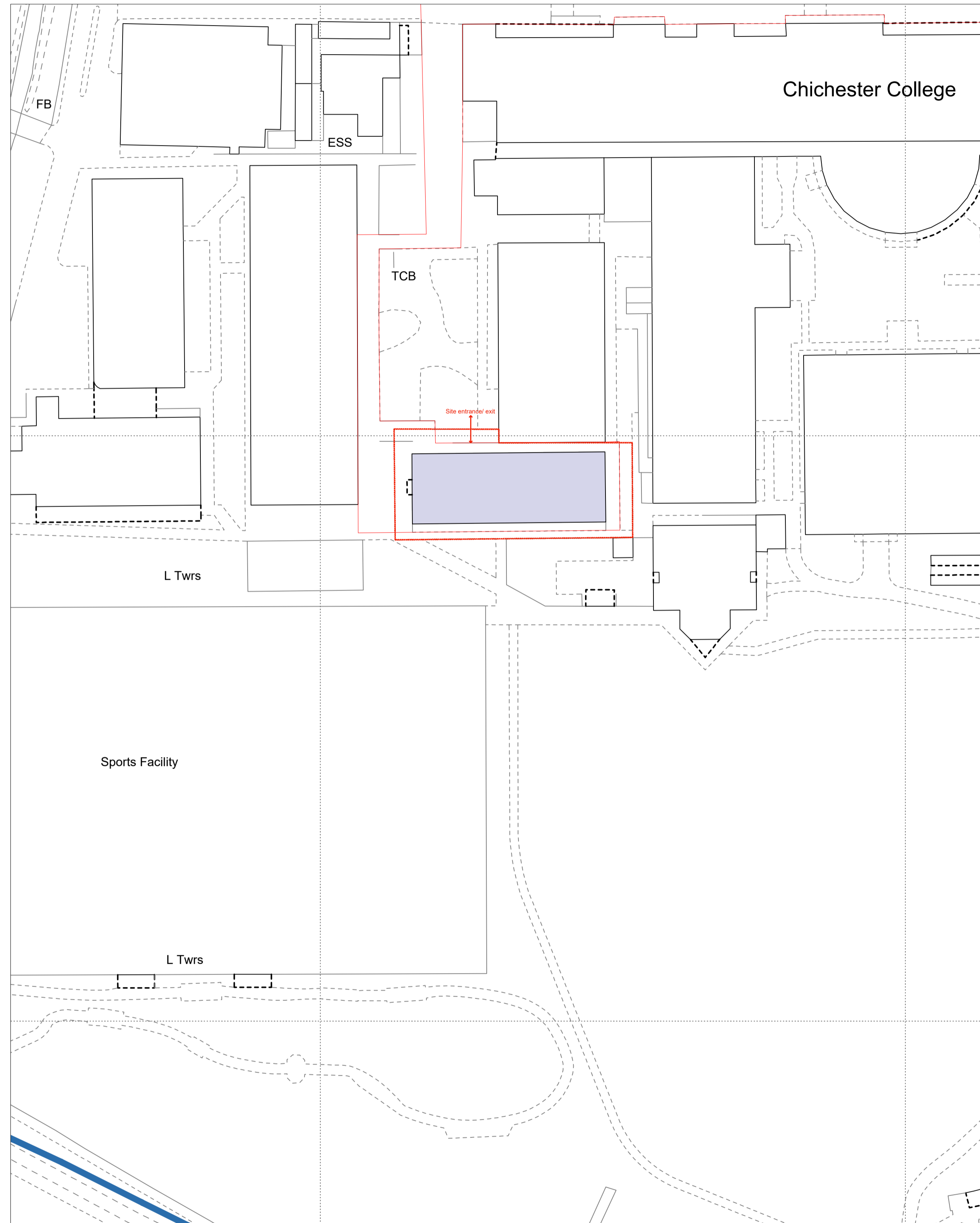
EXISTING BLOCK PLAN SCALE 1:500 @ A1
