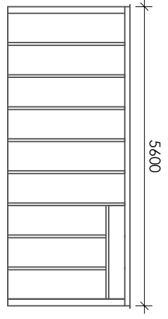
1:100 Front Elevation
