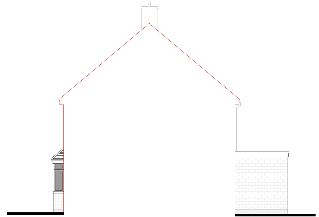
Proposed Side Elevation at 1:50 scale SOUTH WEST
