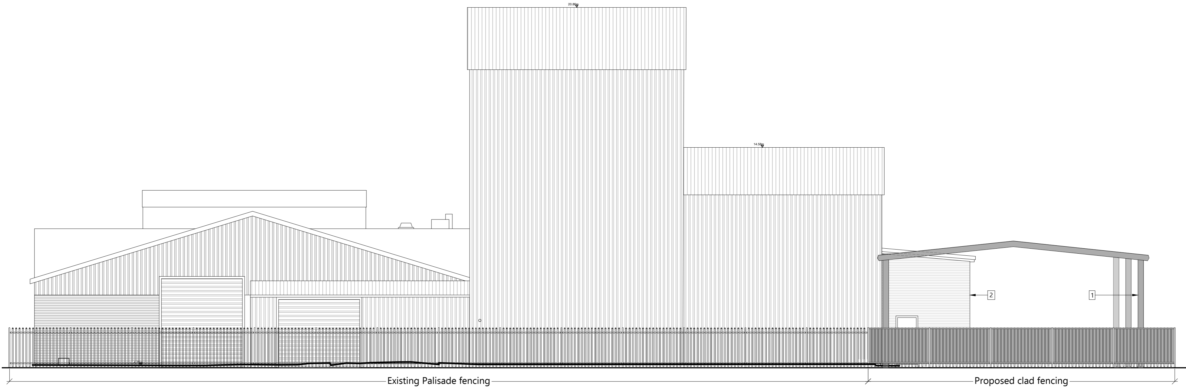
01 Eastern Streetscene Elevation 1:100 0 1m 5m 10m
