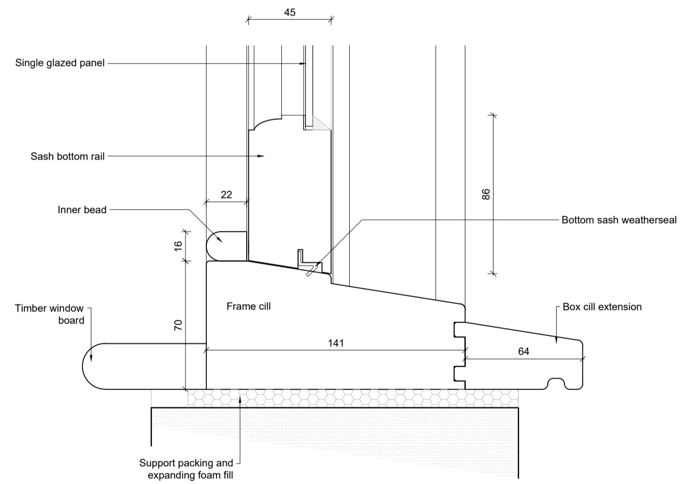
Cill & Head Details
