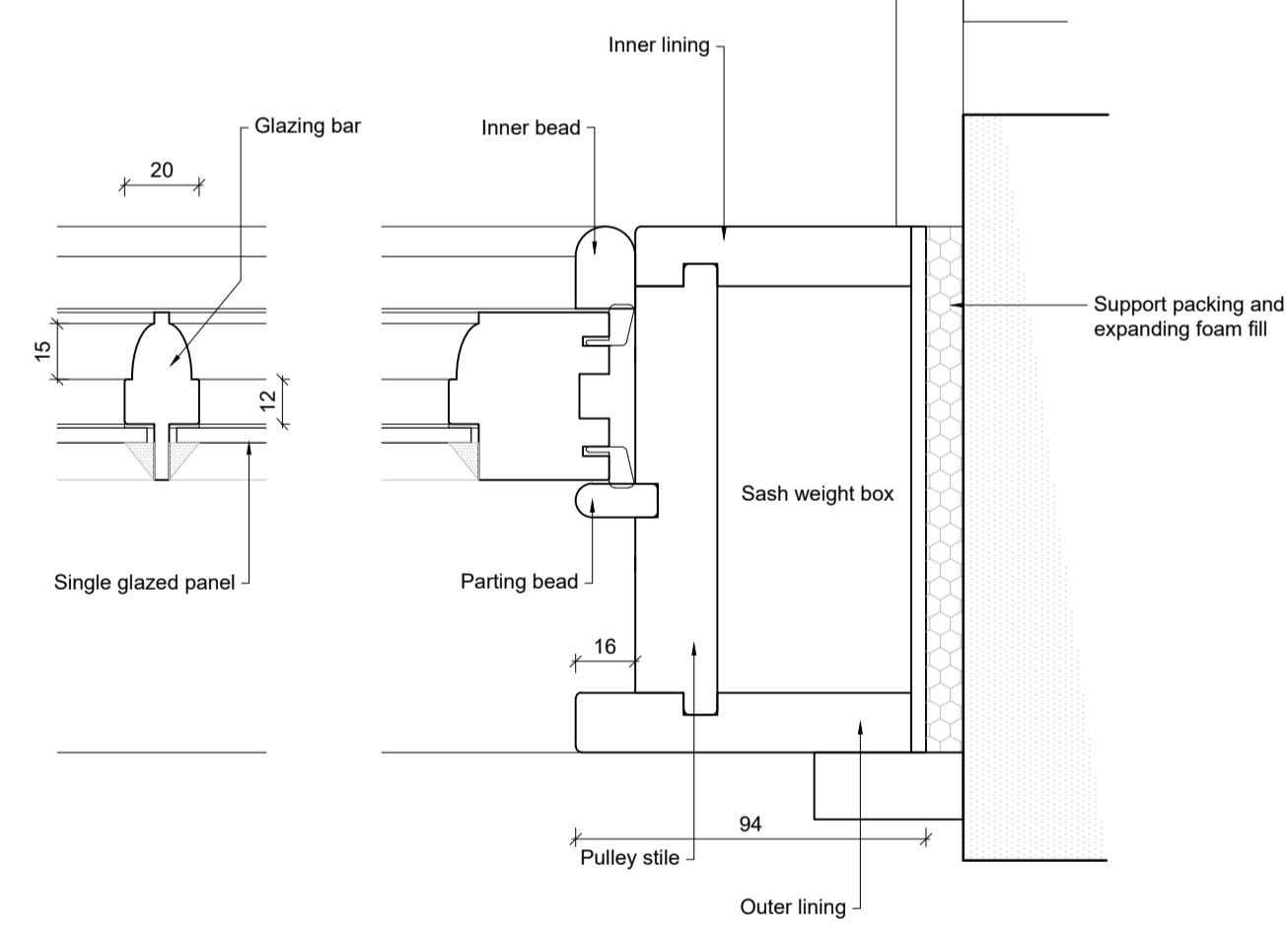
Section B-B
