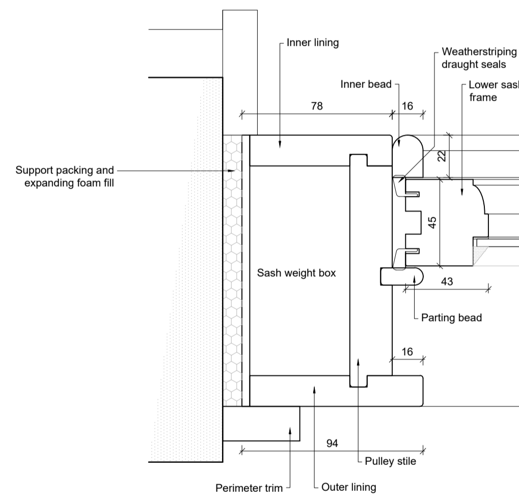
Section B-B
